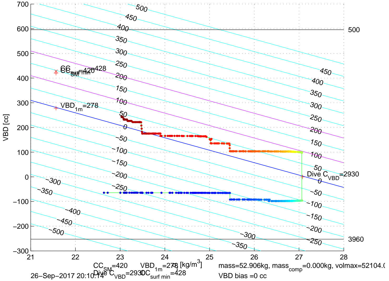
p6100539: SG610 Mission 7 Jul 2017 26-Sep-2017 21:28:06Z – buoyancy contoured
