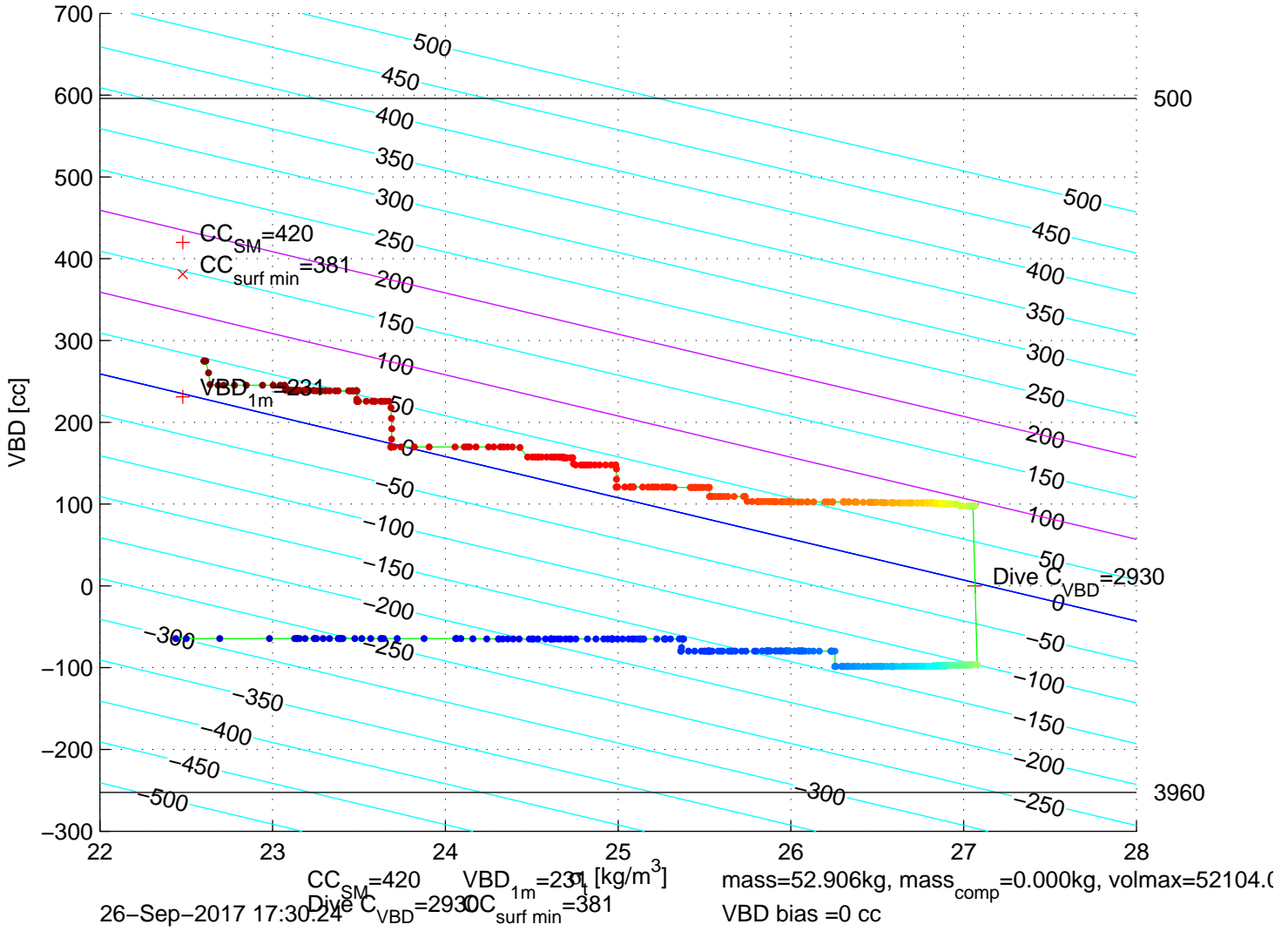
p6100538: SG610 Mission 7 Jul 2017 26-Sep-2017 18:55:24Z – buoyancy contoured
