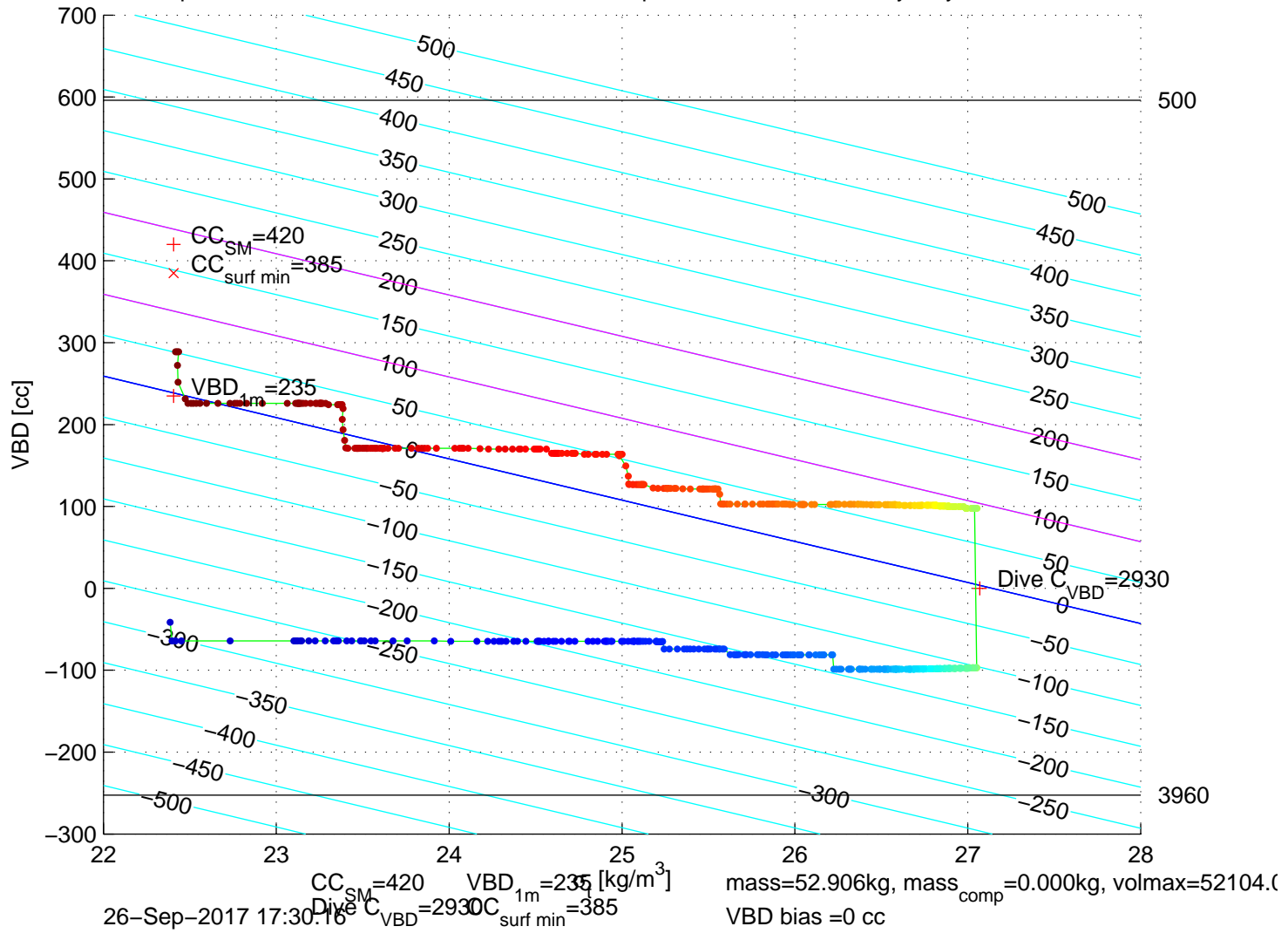
p6100537: SG610 Mission 7 Jul 2017 26-Sep-2017 16:14:31Z – buoyancy contoured
