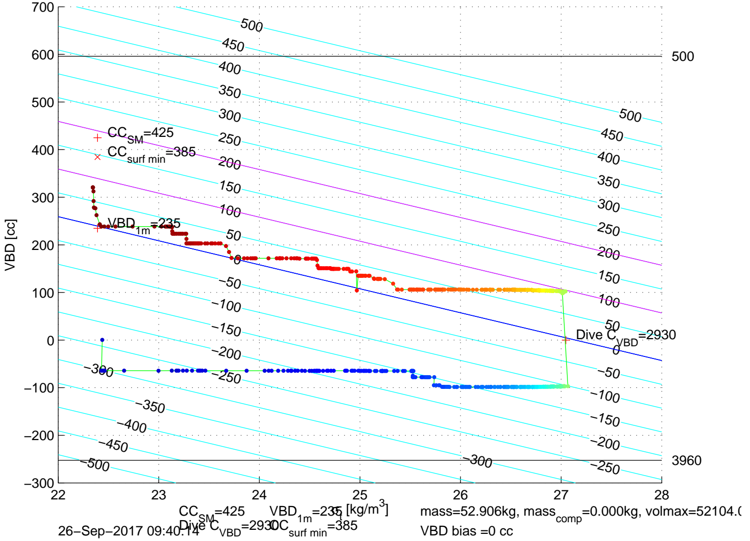
p6100535: SG610 Mission 7 Jul 2017 26-Sep-2017 11:07:47Z – buoyancy contoured
