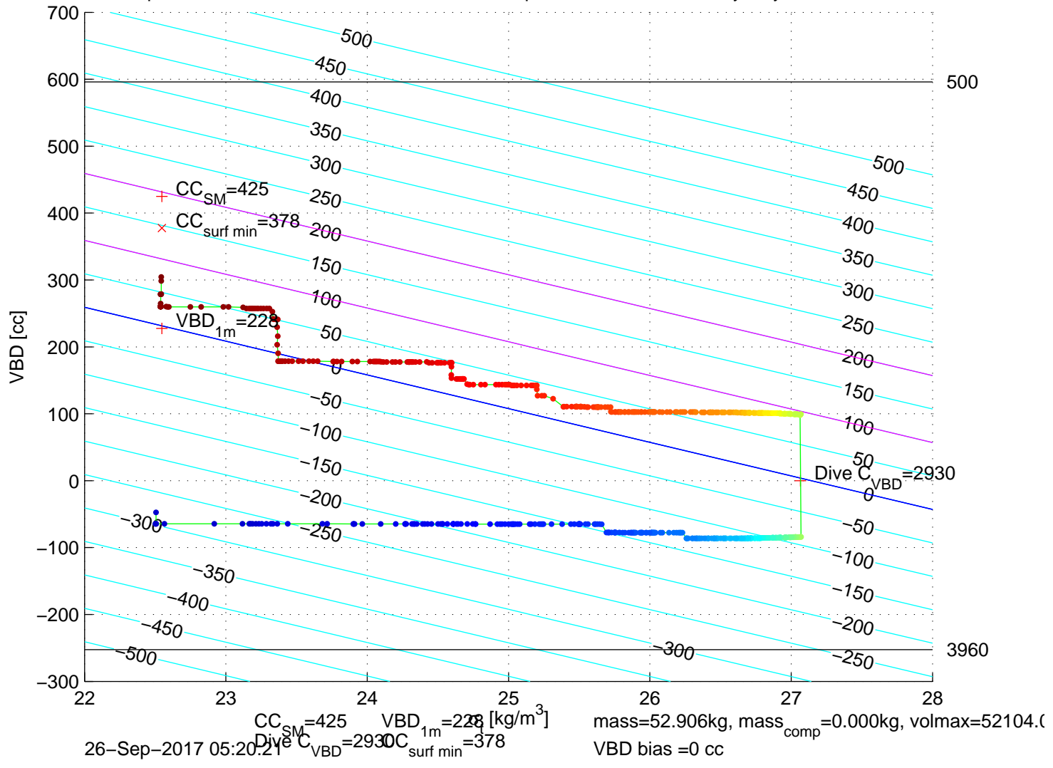
p6100533: SG610 Mission 7 Jul 2017 26-Sep-2017 06:02:19Z – buoyancy contoured
