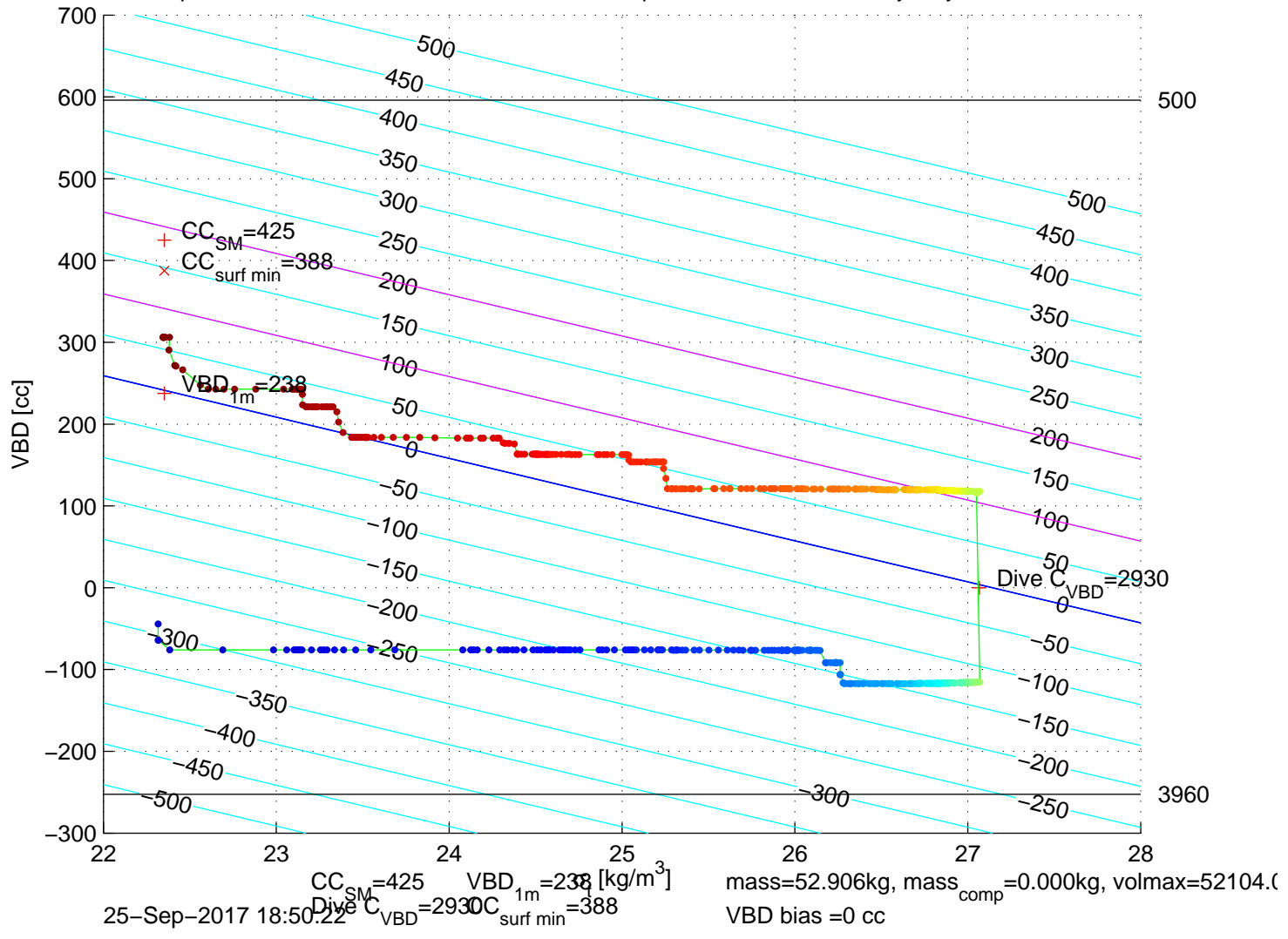
p6100529: SG610 Mission 7 Jul 2017 25-Sep-2017 20:30:52Z – buoyancy contoured
