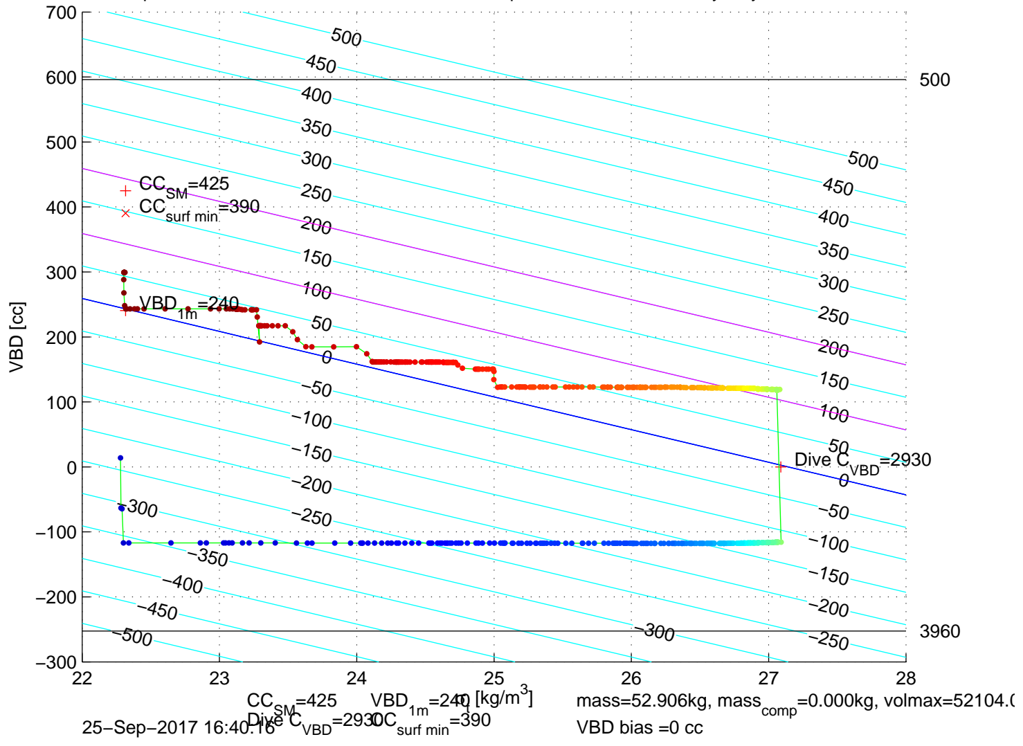
p6100528: SG610 Mission 7 Jul 2017 25-Sep-2017 18:16:43Z – buoyancy contoured
