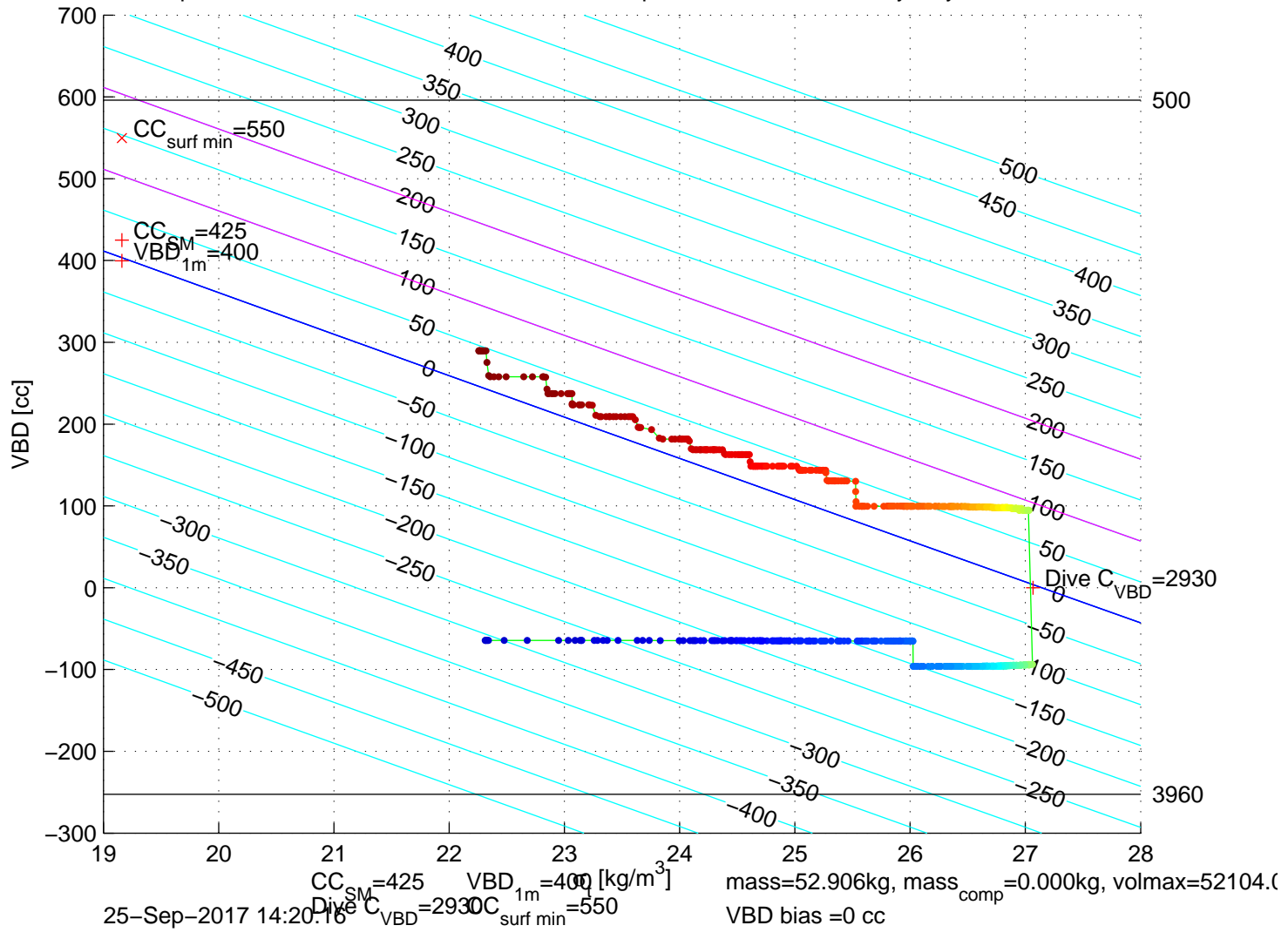
p6100527: SG610 Mission 7 Jul 2017 25-Sep-2017 15:37:30Z – buoyancy contoured
