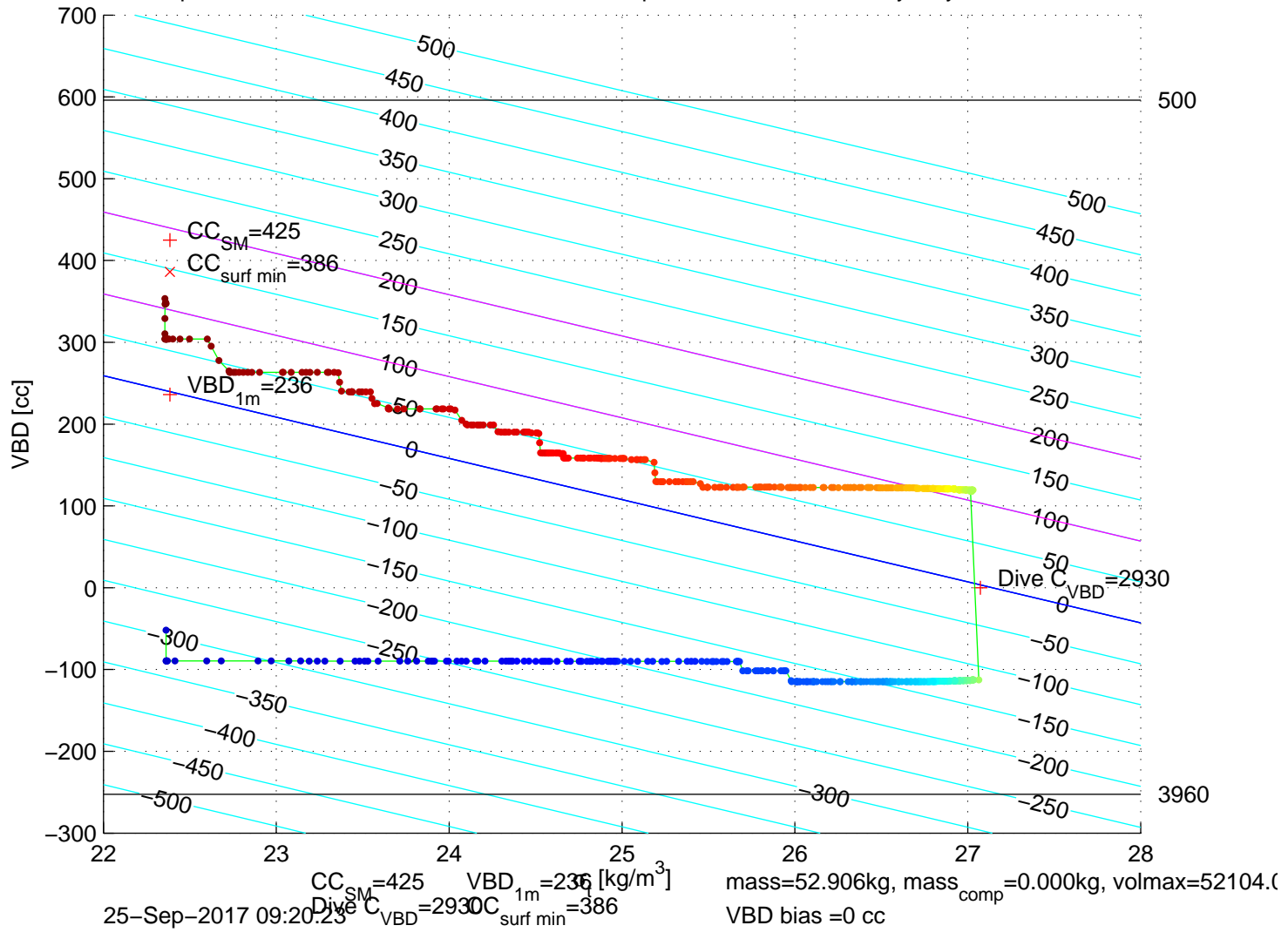
p6100525: SG610 Mission 7 Jul 2017 25-Sep-2017 10:37:57Z – buoyancy contoured
