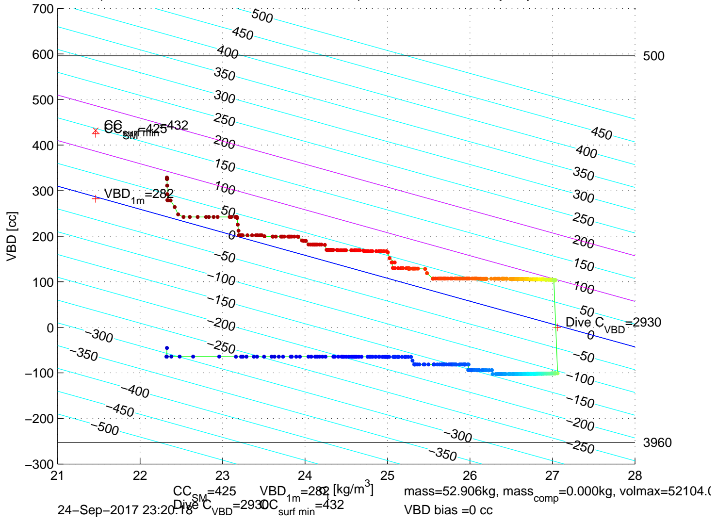
p6100521: SG610 Mission 7 Jul 2017 25-Sep-2017 00:47:04Z – buoyancy contoured
