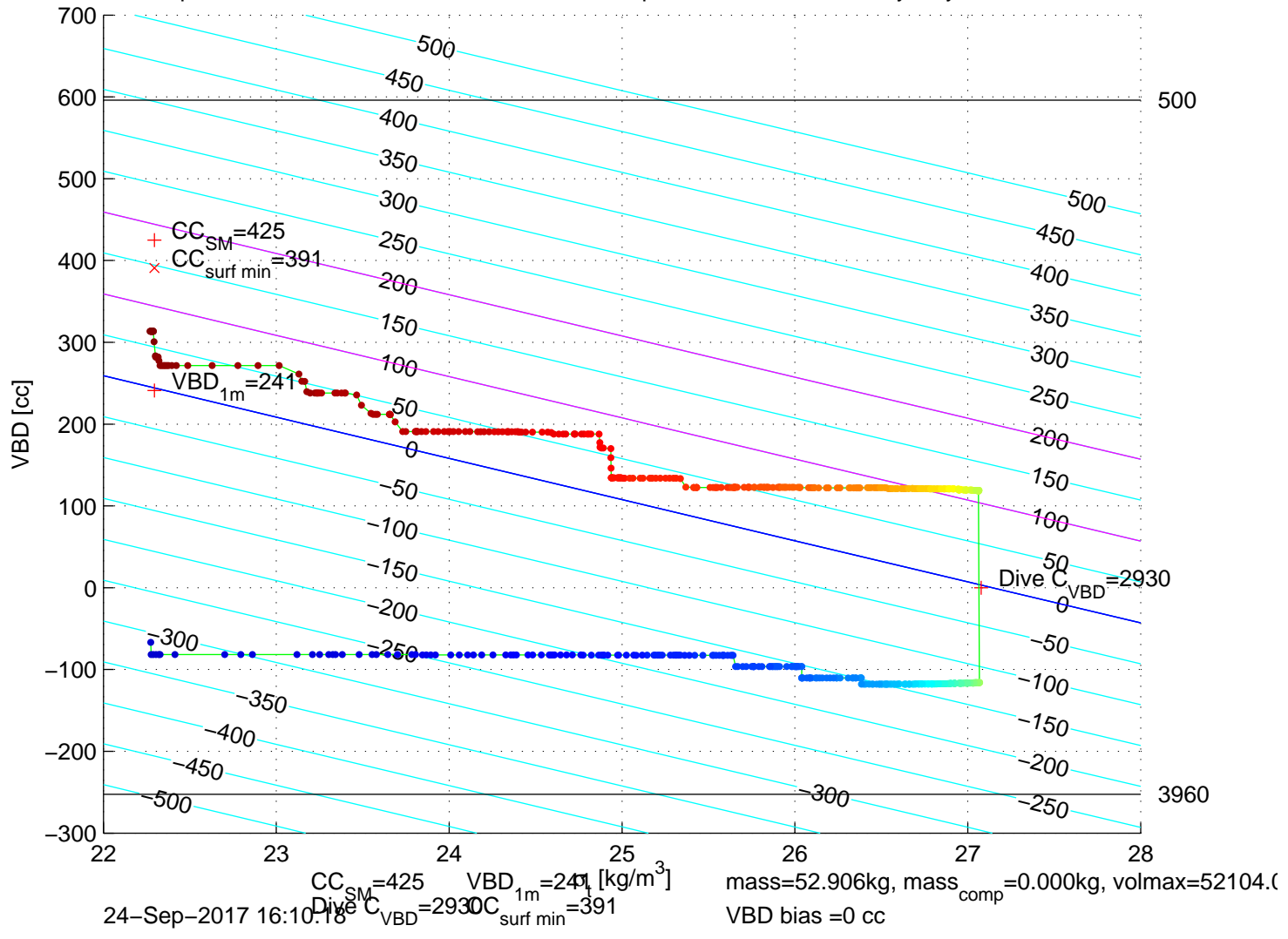
p6100518: SG610 Mission 7 Jul 2017 24-Sep-2017 17:34:15Z – buoyancy contoured
