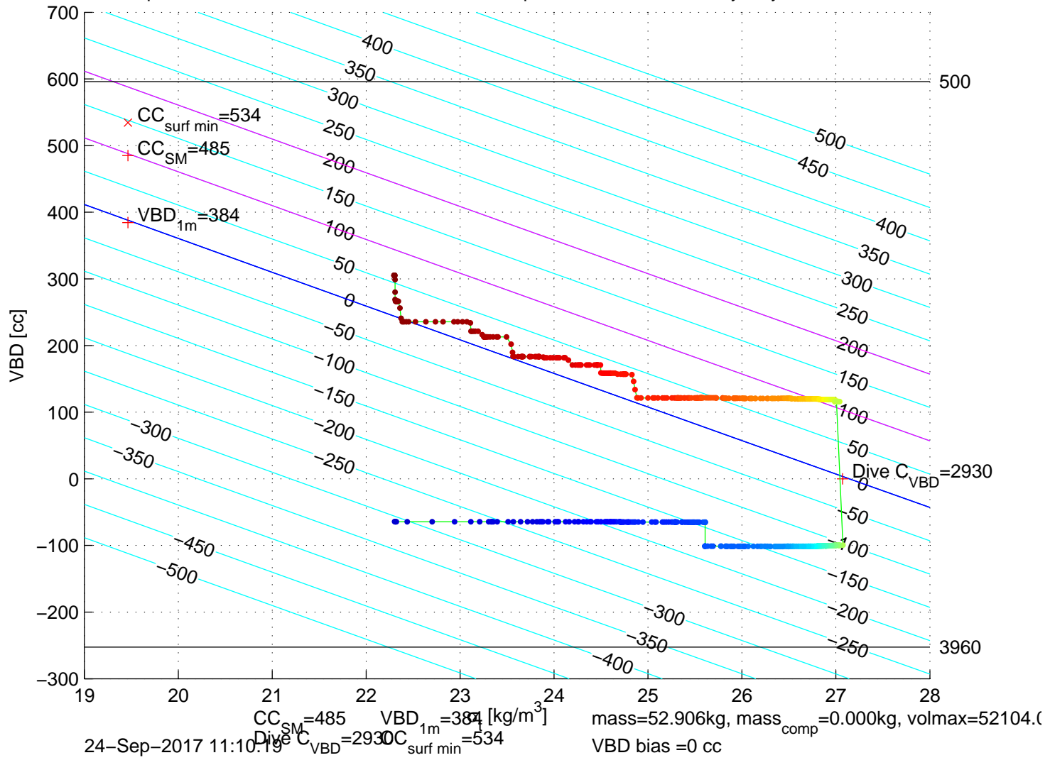
p6100516: SG610 Mission 7 Jul 2017 24-Sep-2017 12:34:31Z - buoyancy contoured
