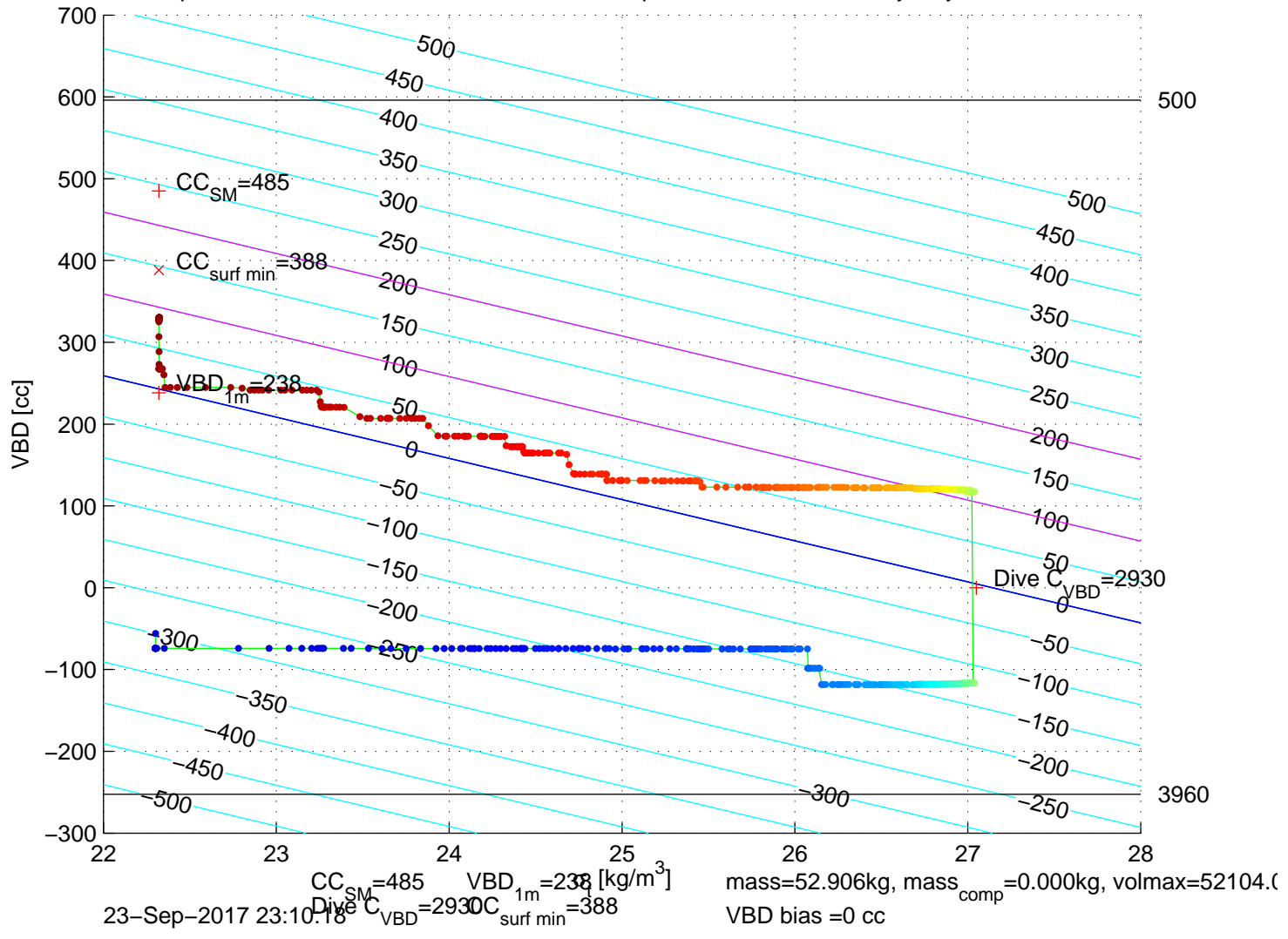
p6100511: SG610 Mission 7 Jul 2017 24-Sep-2017 00:35:20Z – buoyancy contoured
