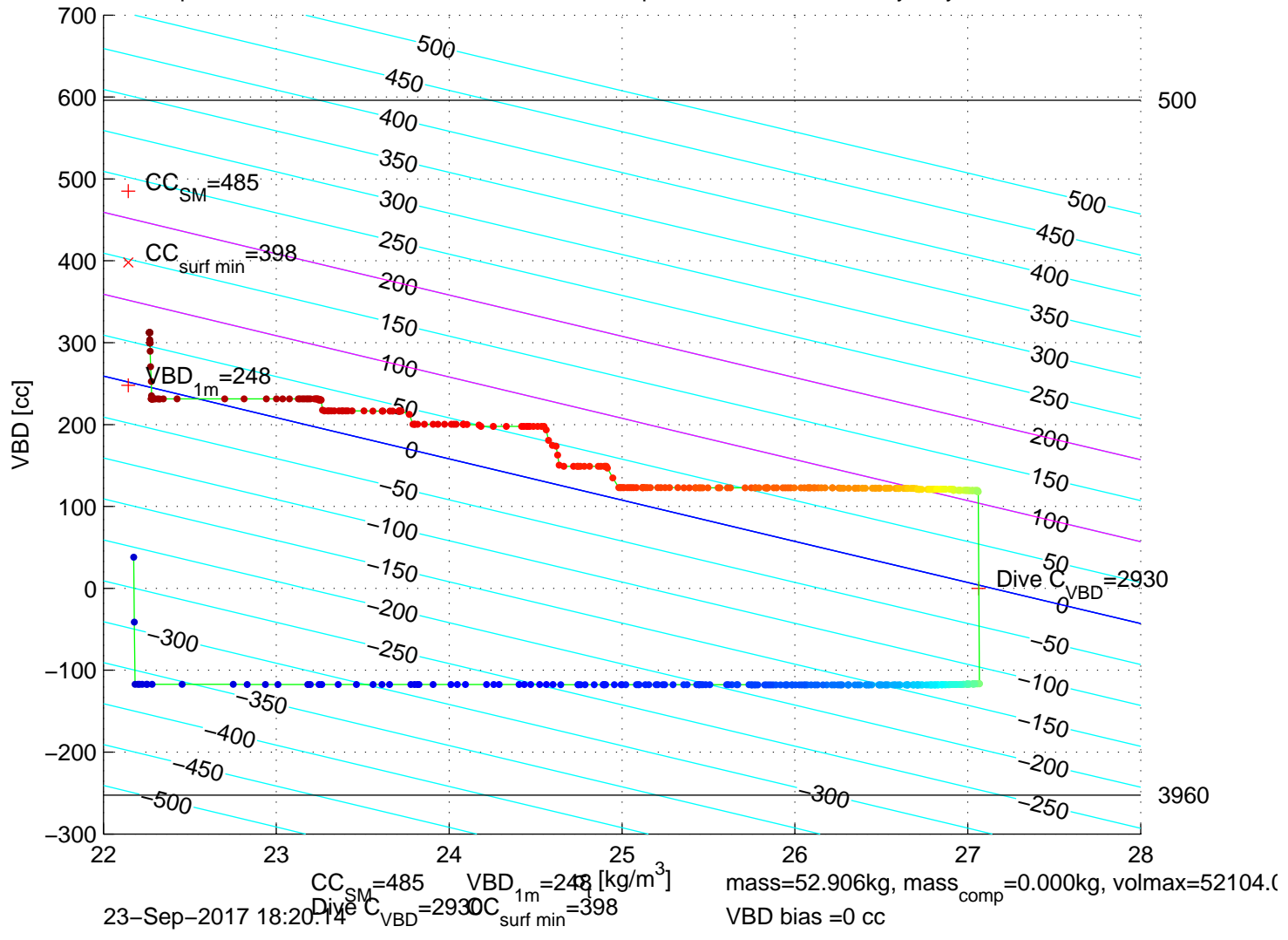
p6100509: SG610 Mission 7 Jul 2017 23-Sep-2017 19:59:43Z – buoyancy contoured
