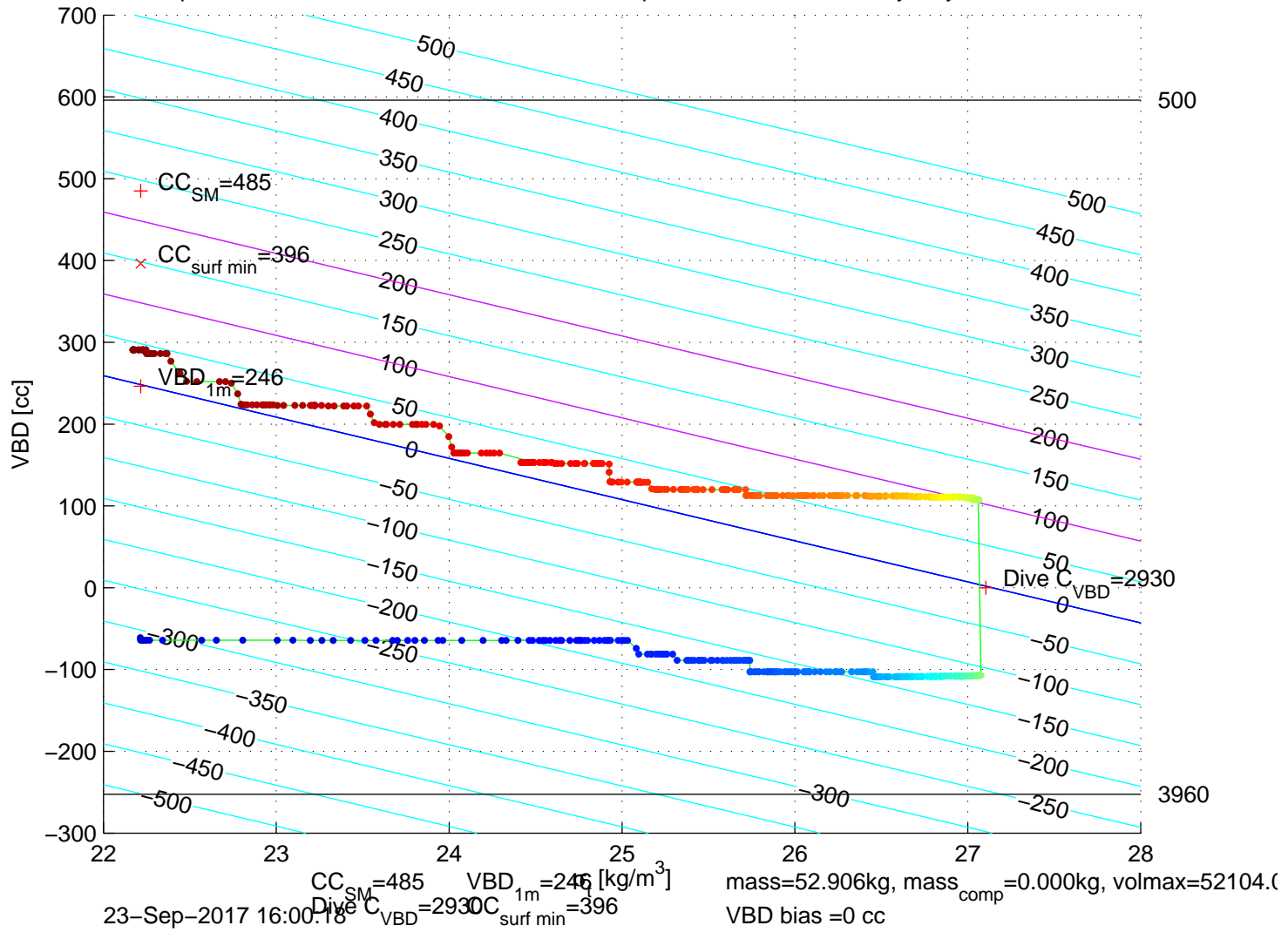
p6100508: SG610 Mission 7 Jul 2017 23-Sep-2017 17:34:58Z – buoyancy contoured
