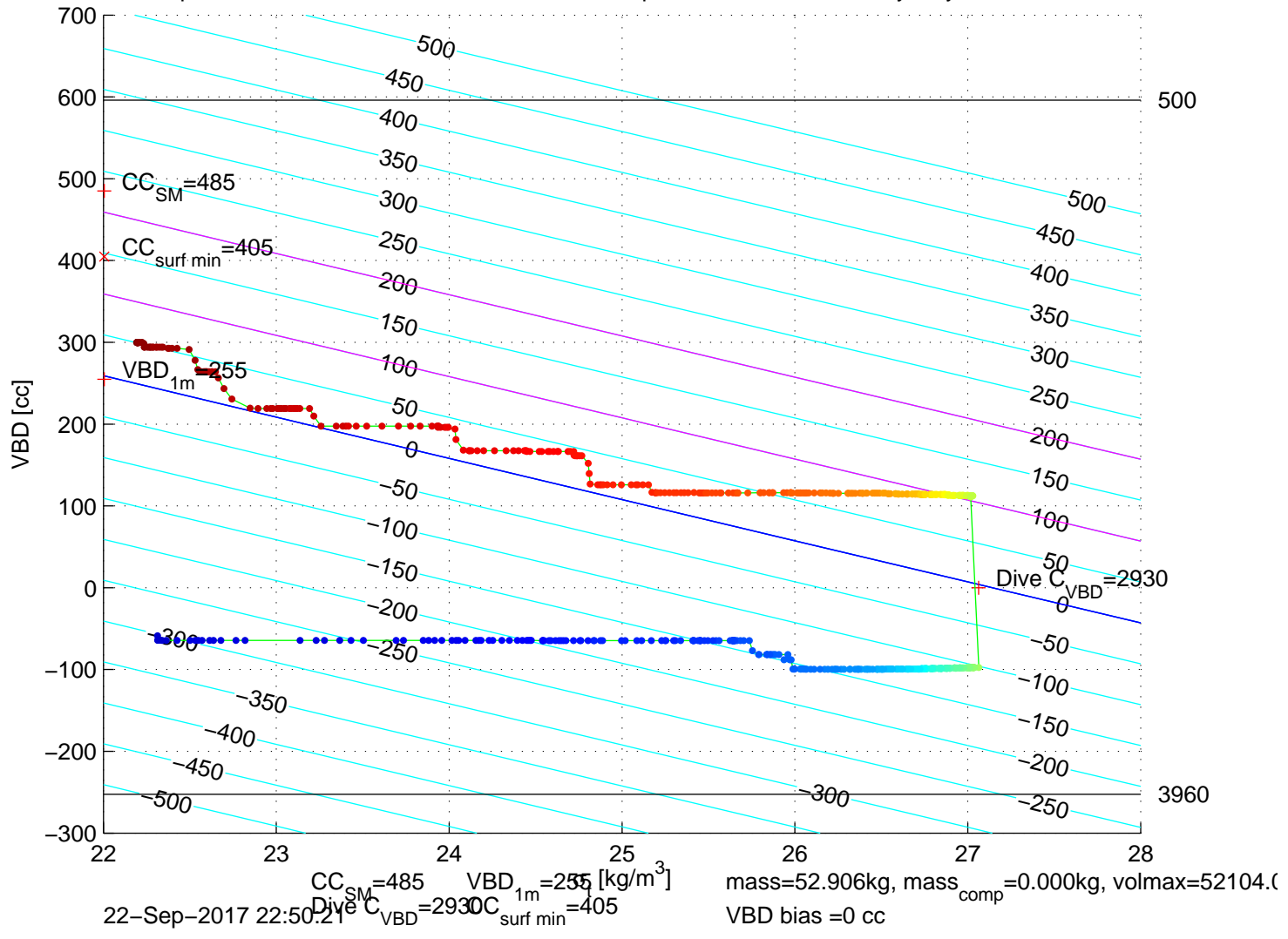
p6100501: SG610 Mission 7 Jul 2017 23-Sep-2017 00:19:13Z – buoyancy contoured
