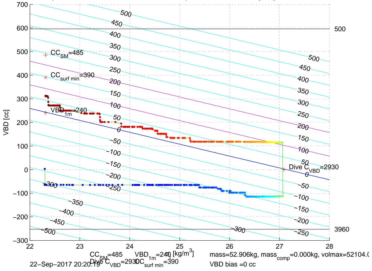
p6100500: SG610 Mission 7 Jul 2017 22-Sep-2017 21:54:27Z – buoyancy contoured
