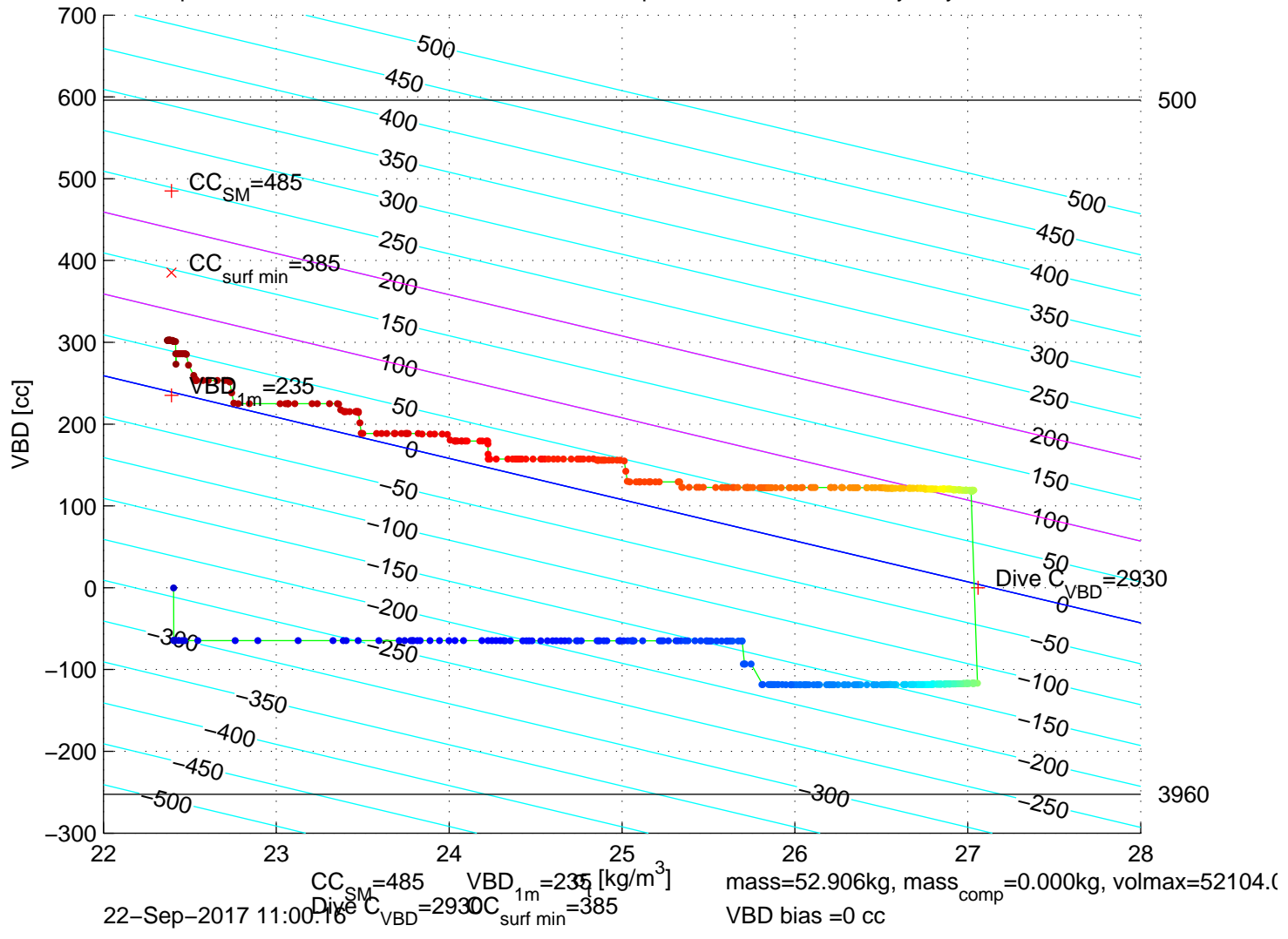
p6100496: SG610 Mission 7 Jul 2017 22-Sep-2017 12:35:00Z – buoyancy contoured
