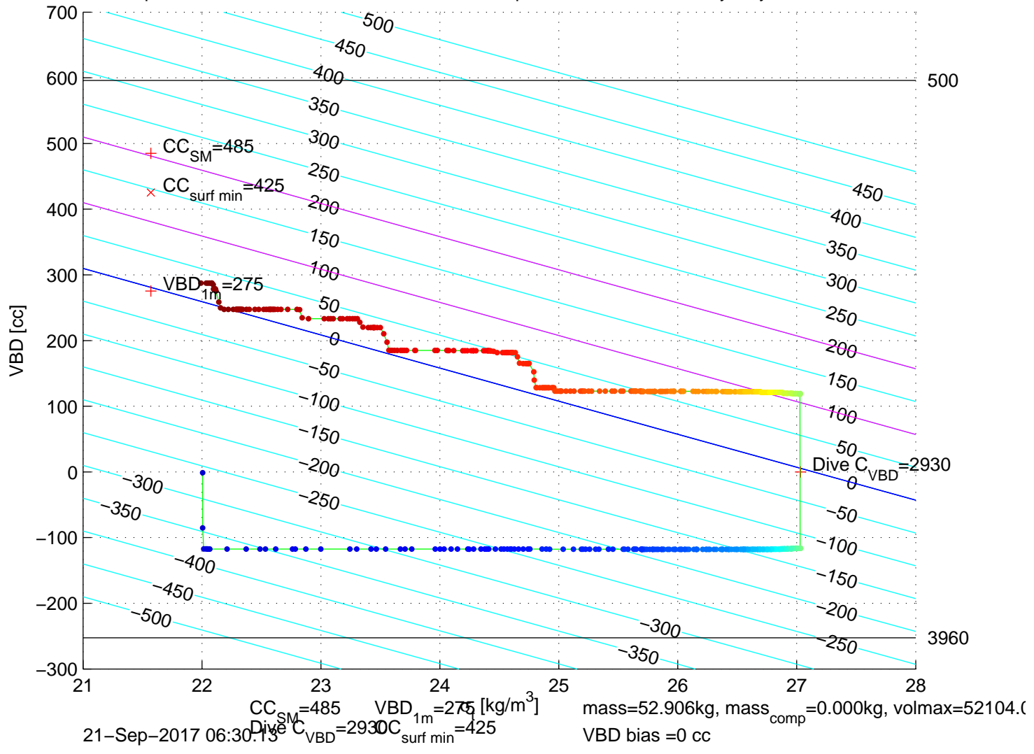
p6100484: SG610 Mission 7 Jul 2017 21-Sep-2017 08:09:13Z – buoyancy contoured
