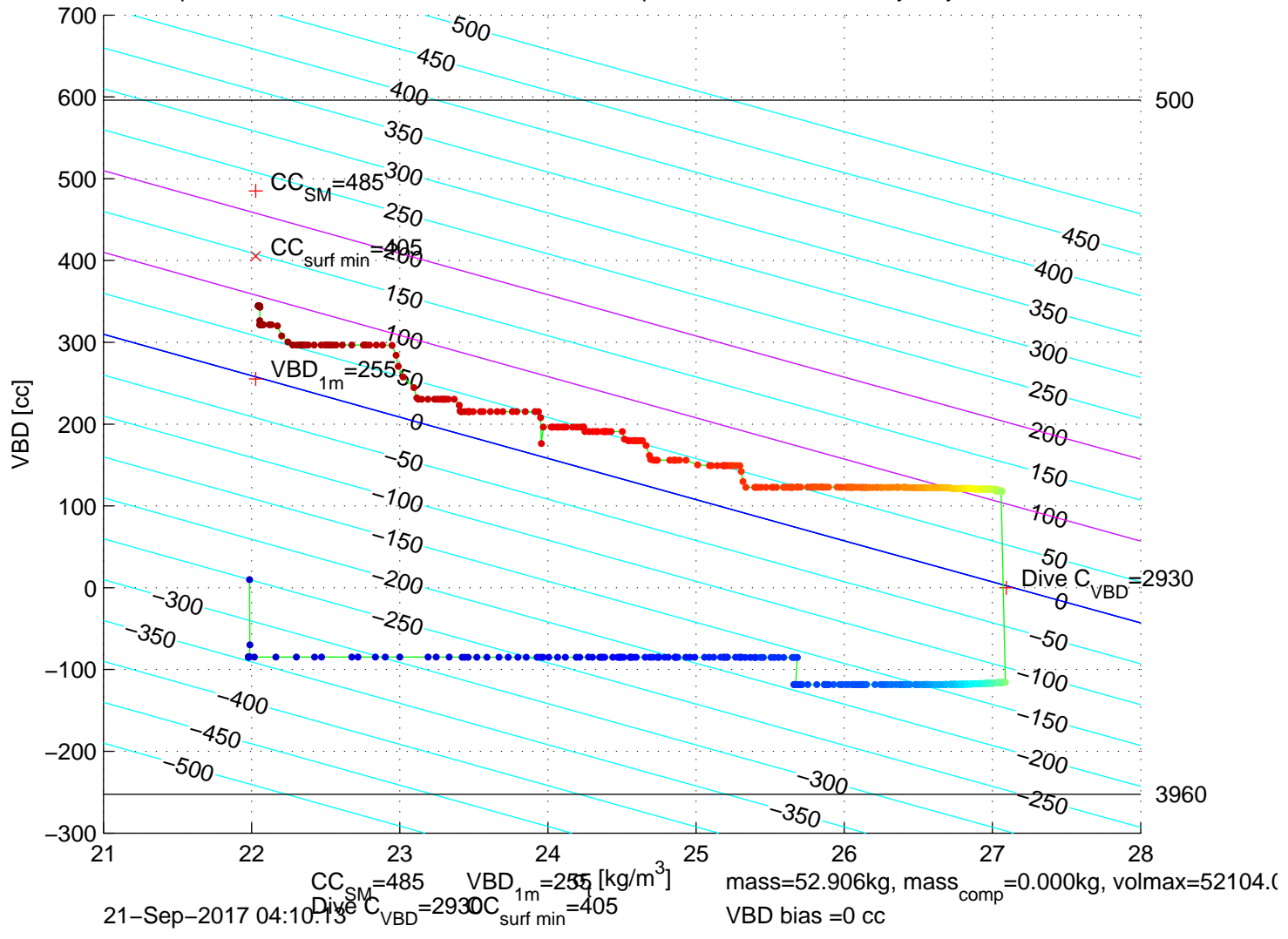
p6100483: SG610 Mission 7 Jul 2017 21-Sep-2017 05:30:28Z – buoyancy contoured
