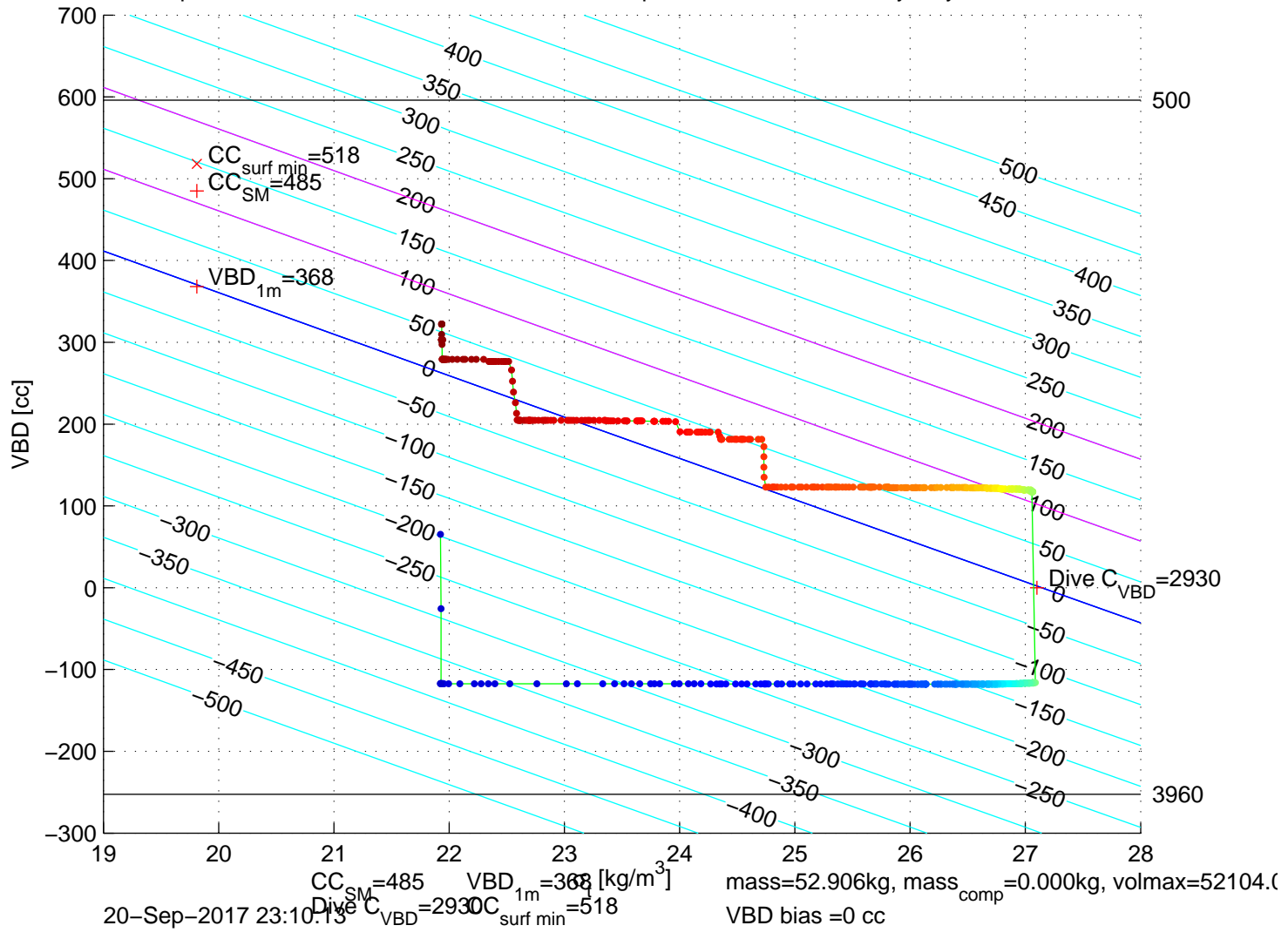
p6100481: SG610 Mission 7 Jul 2017 21-Sep-2017 00:44:54Z – buoyancy contoured
