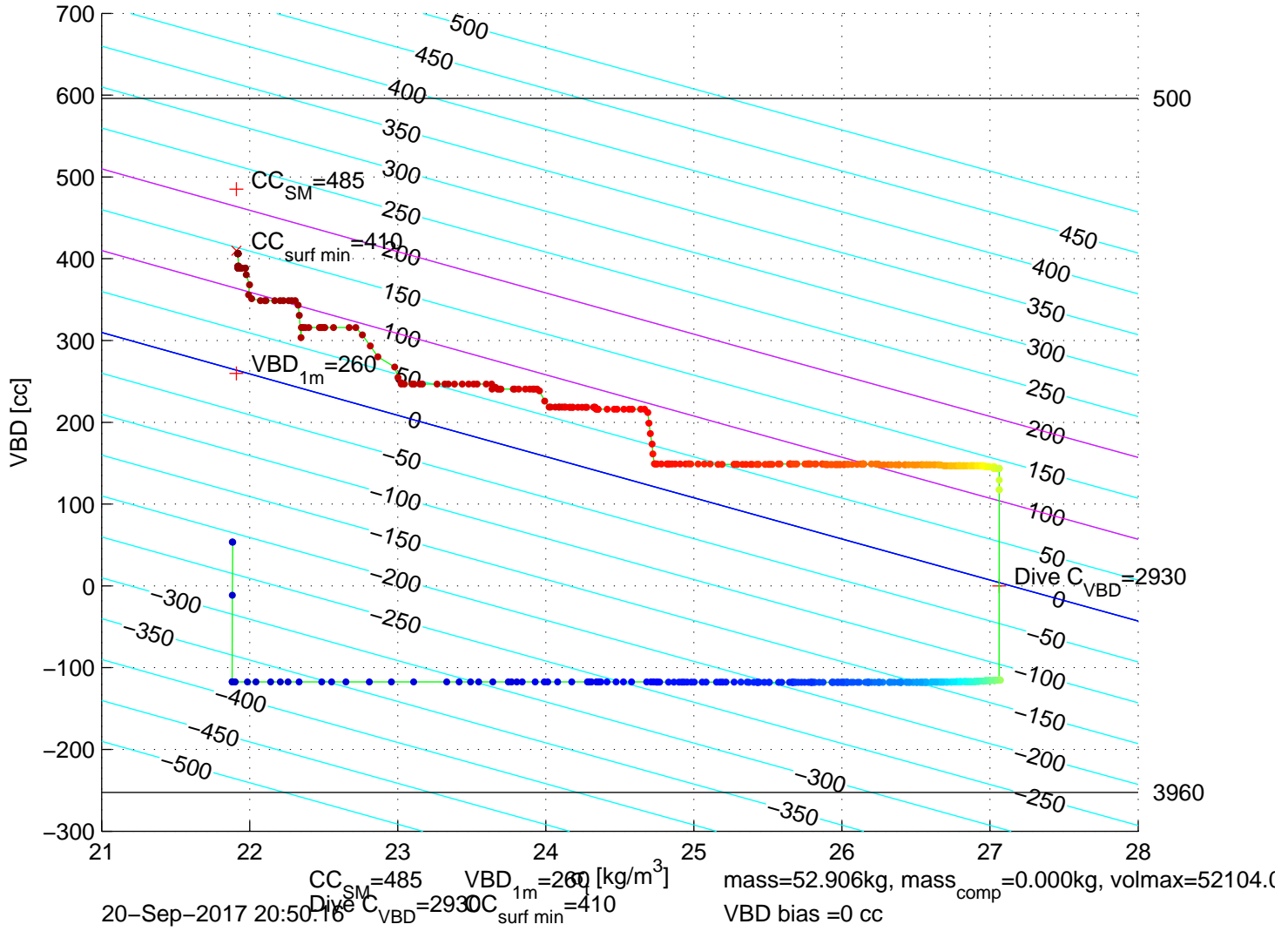
p6100480: SG610 Mission 7 Jul 2017 20-Sep-2017 22:10:15Z – buoyancy contoured
