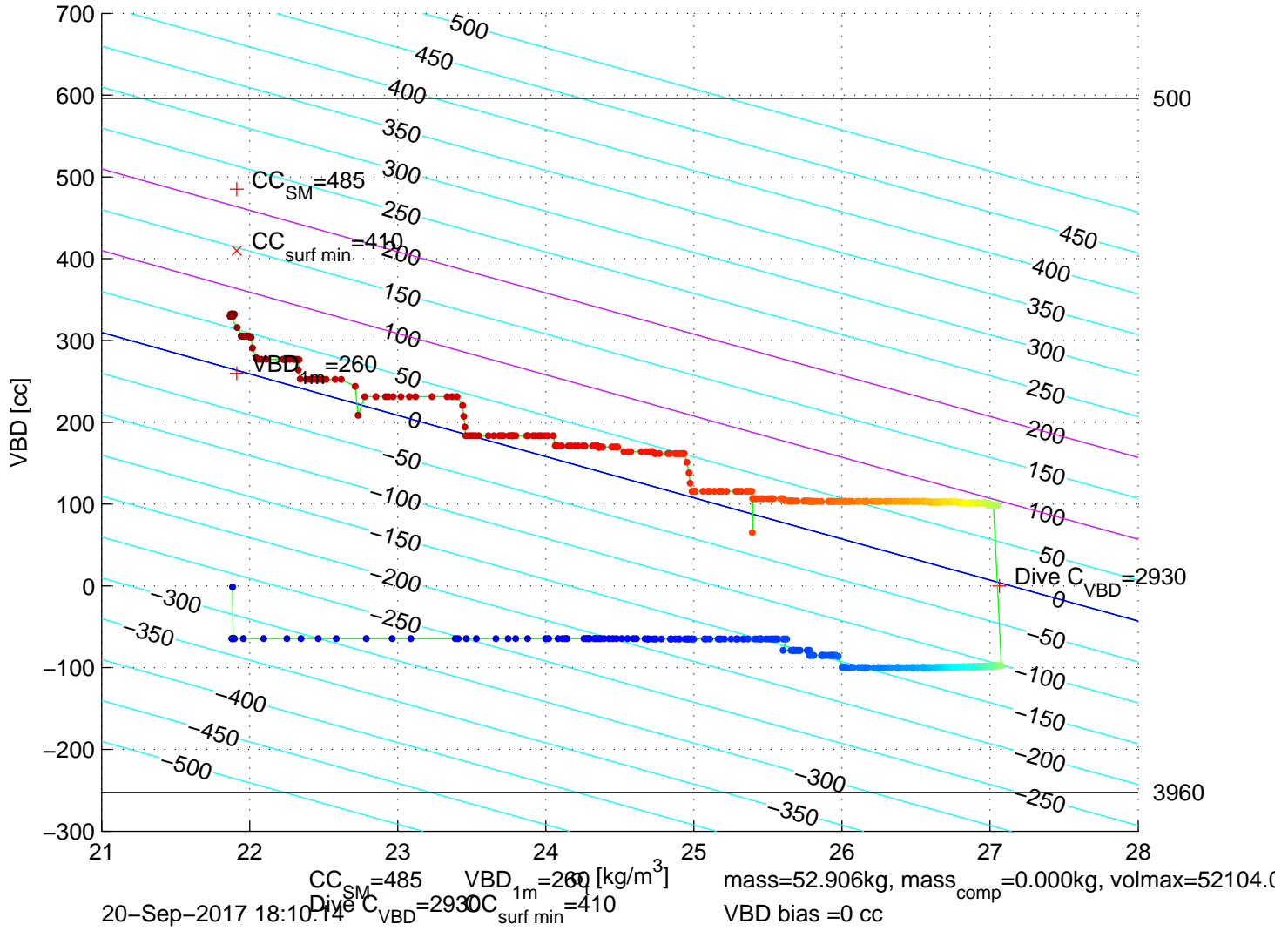
p6100479: SG610 Mission 7 Jul 2017 20-Sep-2017 19:37:29Z – buoyancy contoured
