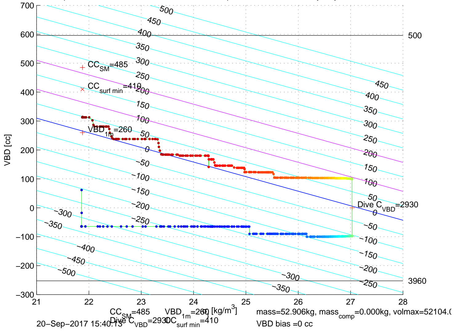
p6100478: SG610 Mission 7 Jul 2017 20-Sep-2017 17:07:12Z – buoyancy contoured
