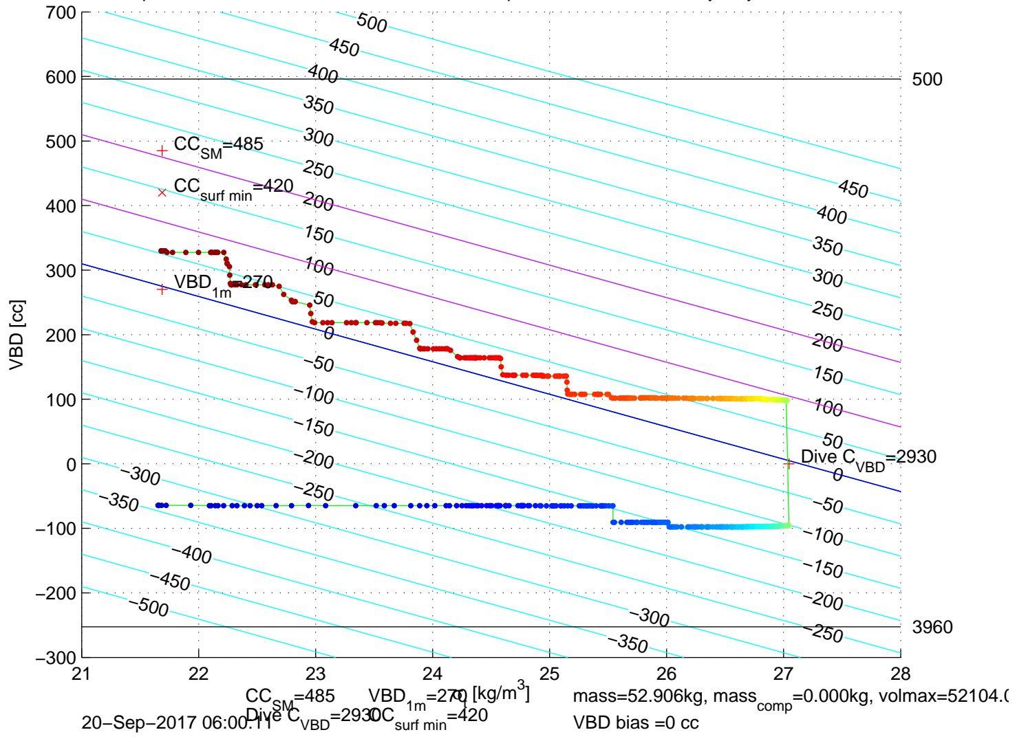
p6100474: SG610 Mission 7 Jul 2017 20-Sep-2017 07:31:59Z – buoyancy contoured
