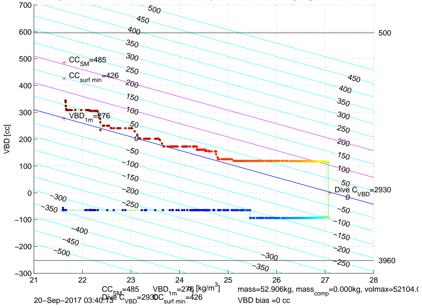
p6100473: SG610 Mission 7 Jul 2017 20-Sep-2017 05:01:57Z – buoyancy contoured
