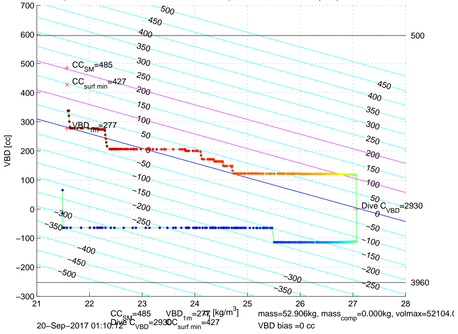
p6100472: SG610 Mission 7 Jul 2017 20-Sep-2017 02:33:29Z – buoyancy contoured
