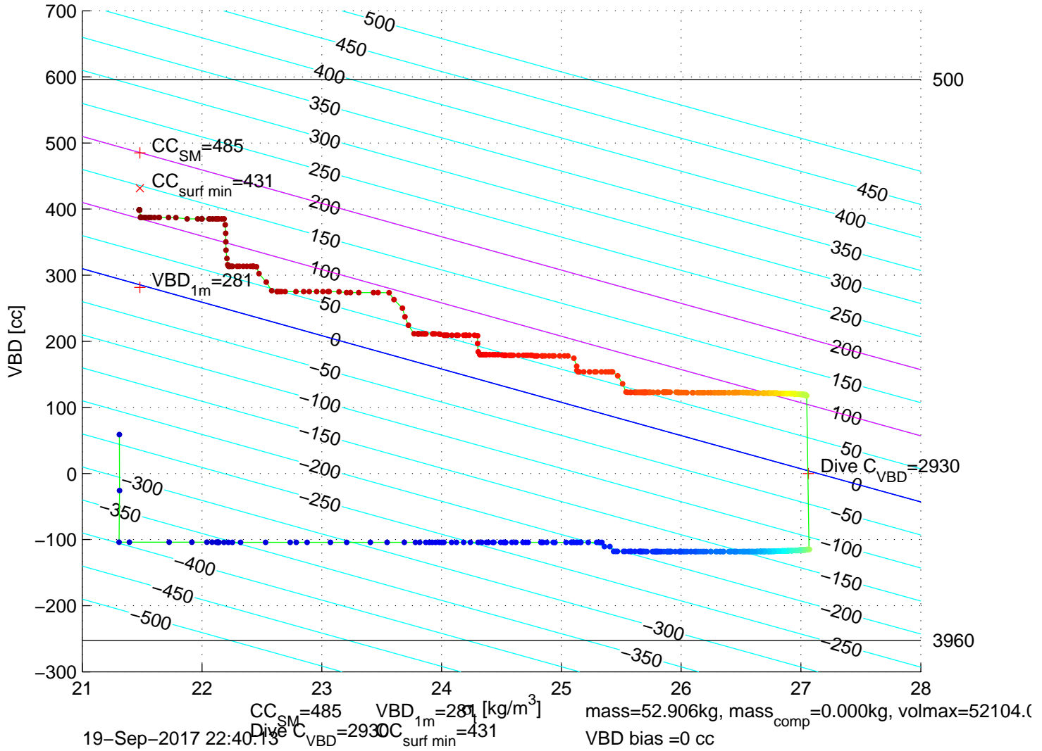
p6100471: SG610 Mission 7 Jul 2017 19-Sep-2017 23:58:09Z – buoyancy contoured
