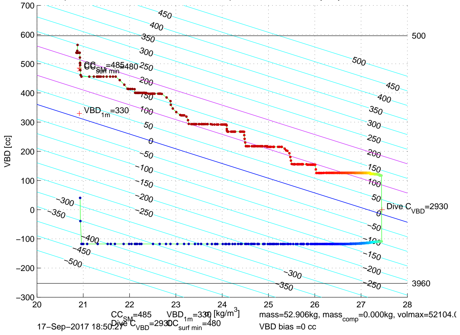
p6100454: SG610 Mission 7 Jul 2017 17-Sep-2017 18:06:12Z – buoyancy contoured
