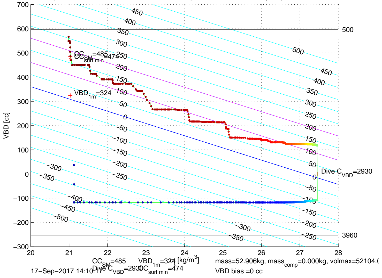
p6100453: SG610 Mission 7 Jul 2017 17-Sep-2017 13:19:46Z – buoyancy contoured
