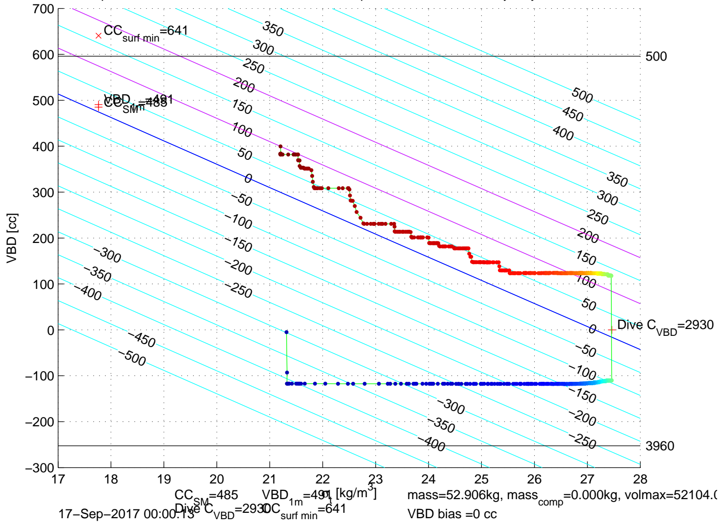
p6100450: SG610 Mission 7 Jul 2017 17-Sep-2017 00:08:57Z – buoyancy contoured
