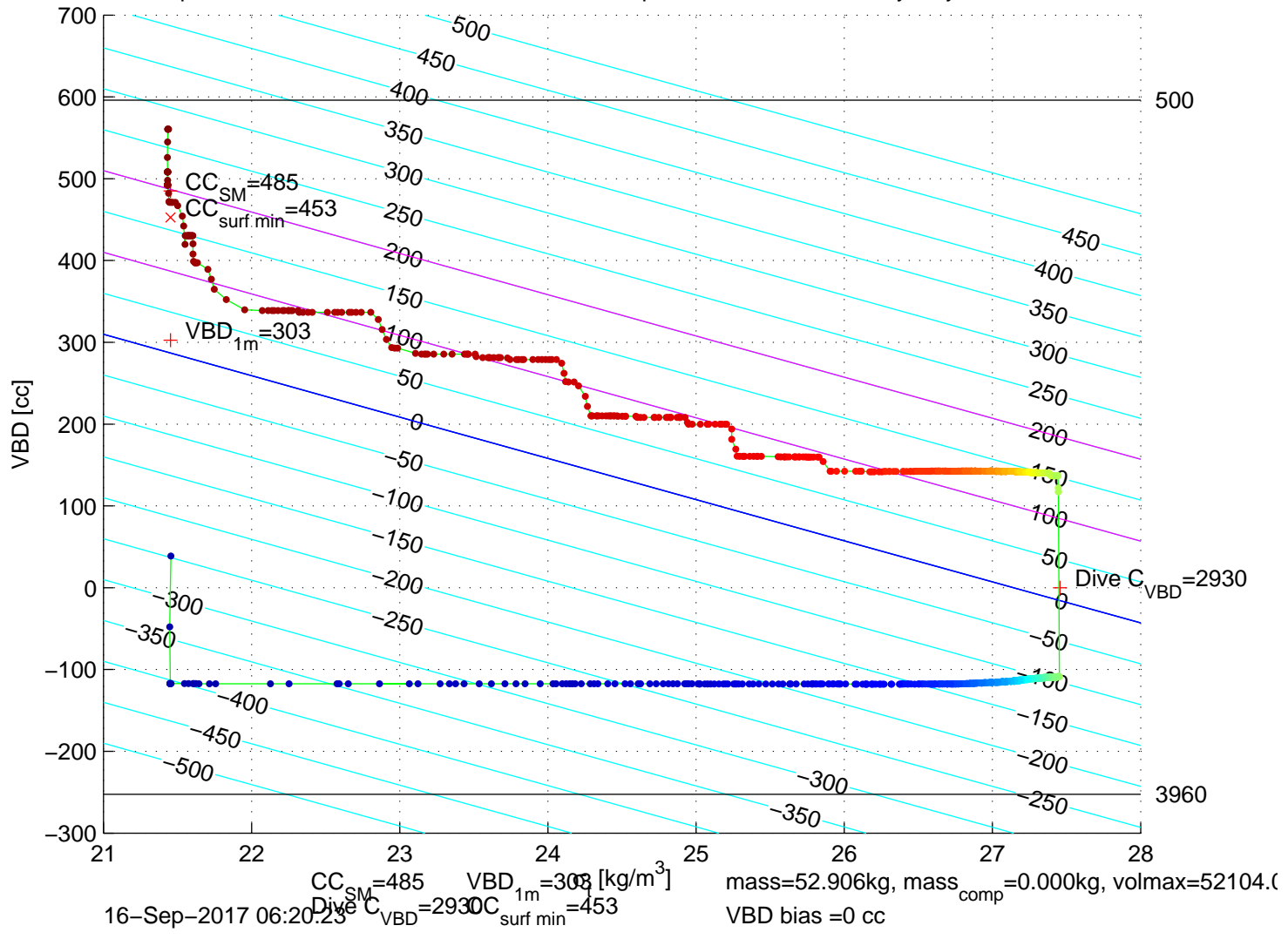
p6100446: SG610 Mission 7 Jul 2017 16-Sep-2017 05:36:12Z – buoyancy contoured
