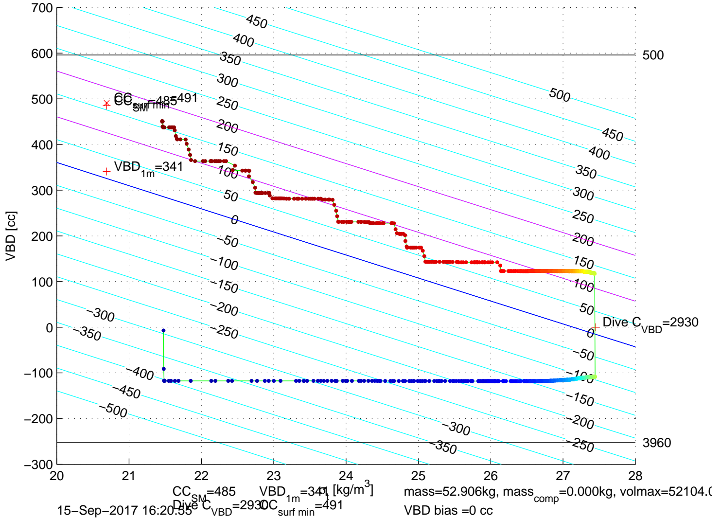
p6100443: SG610 Mission 7 Jul 2017 15-Sep-2017 15:33:08Z – buoyancy contoured
