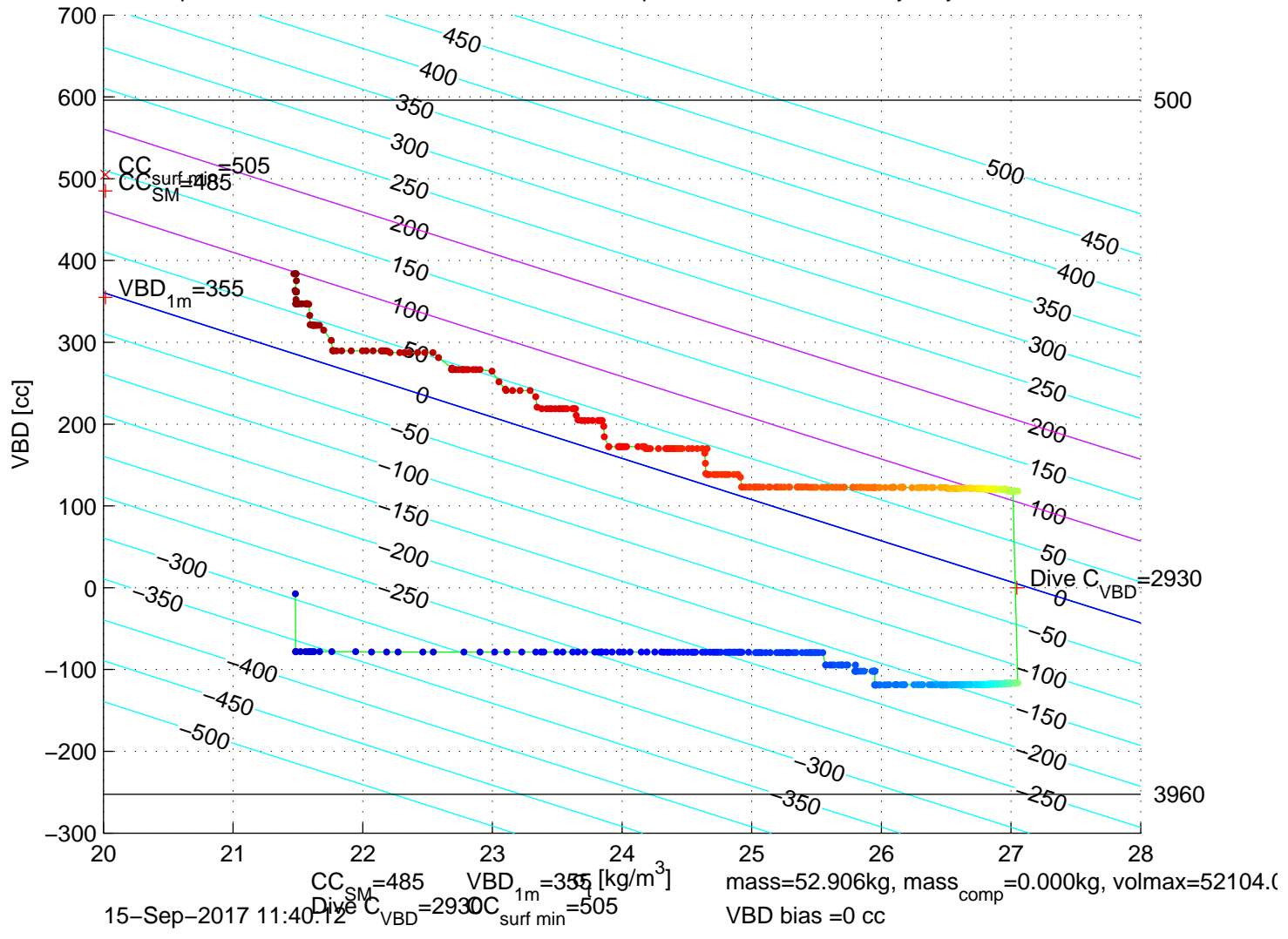
p6100442: SG610 Mission 7 Jul 2017 15-Sep-2017 13:11:02Z – buoyancy contoured
