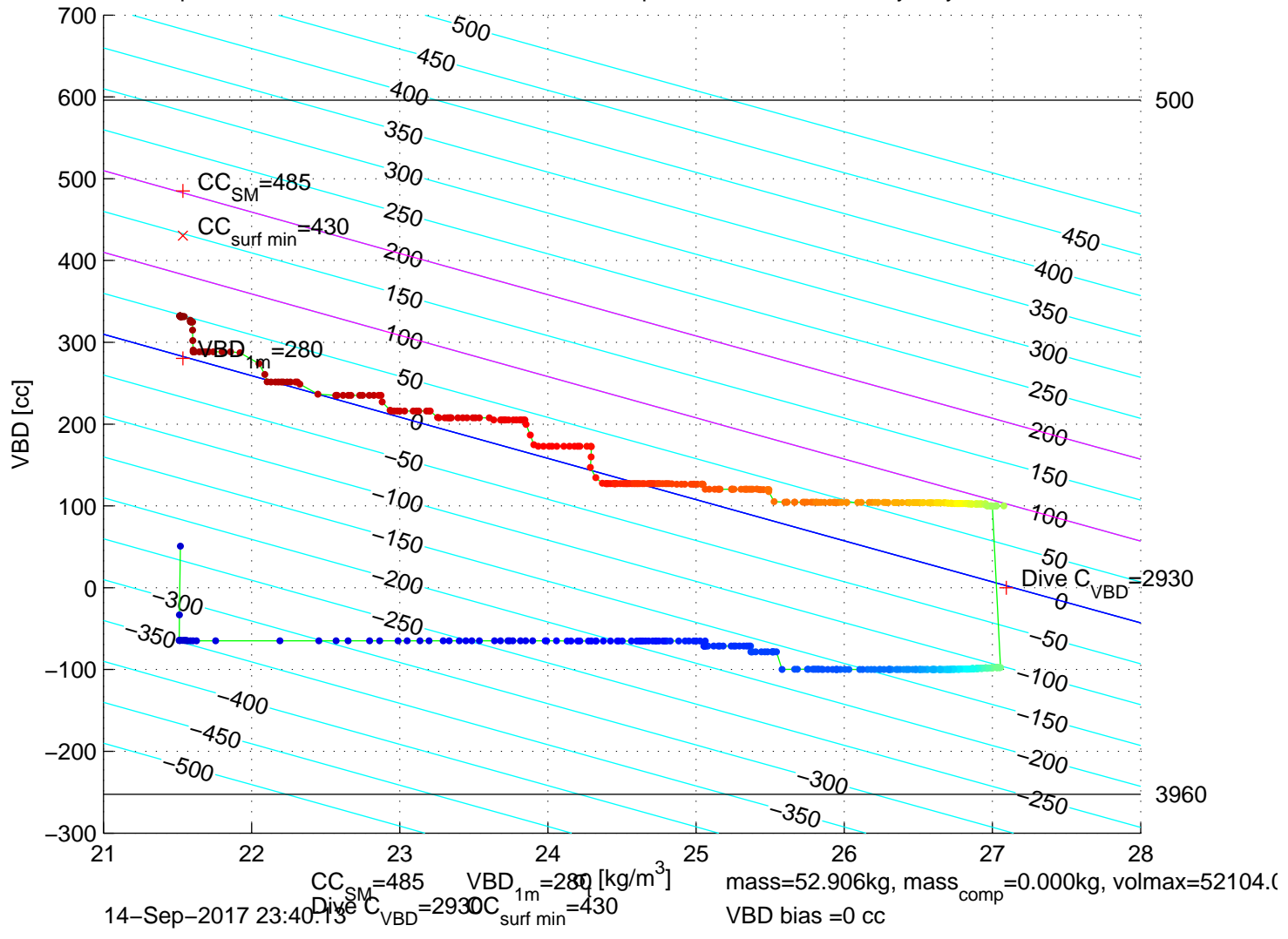
p6100437: SG610 Mission 7 Jul 2017 15-Sep-2017 01:05:26Z – buoyancy contoured
