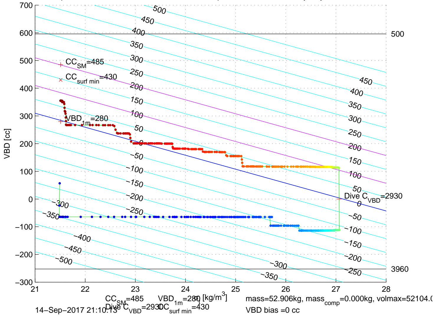
p6100436: SG610 Mission 7 Jul 2017 14-Sep-2017 22:45:39Z – buoyancy contoured
