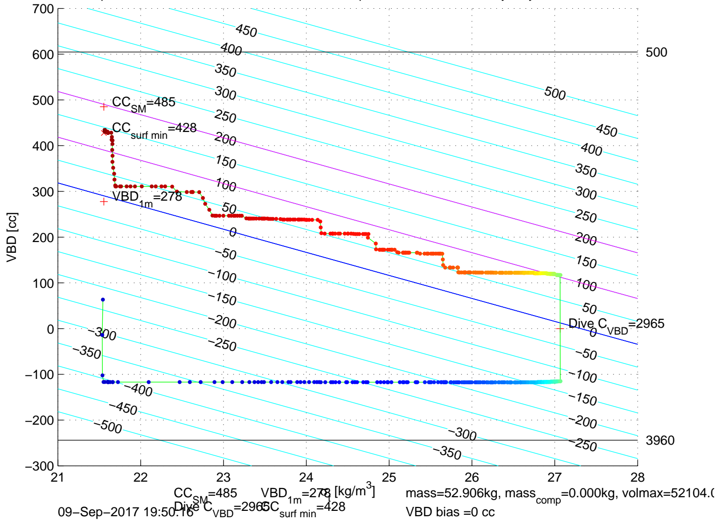
p6100386: SG610 Mission 7 Jul 2017 09-Sep-2017 21:08:49Z – buoyancy contoured
