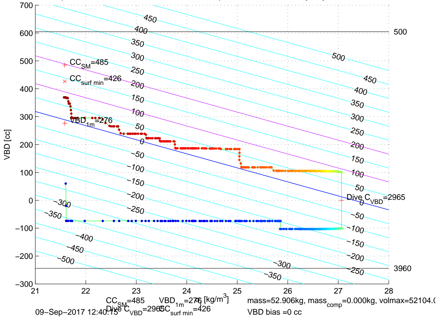
p6100383: SG610 Mission 7 Jul 2017 09-Sep-2017 14:05:08Z – buoyancy contoured
