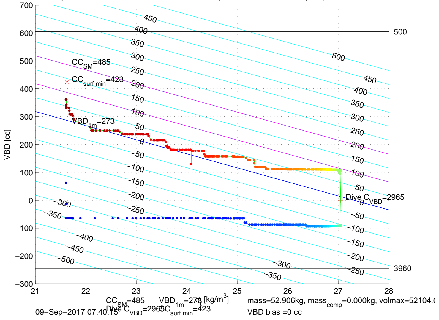
p6100381: SG610 Mission 7 Jul 2017 09-Sep-2017 09:10:56Z – buoyancy contoured
