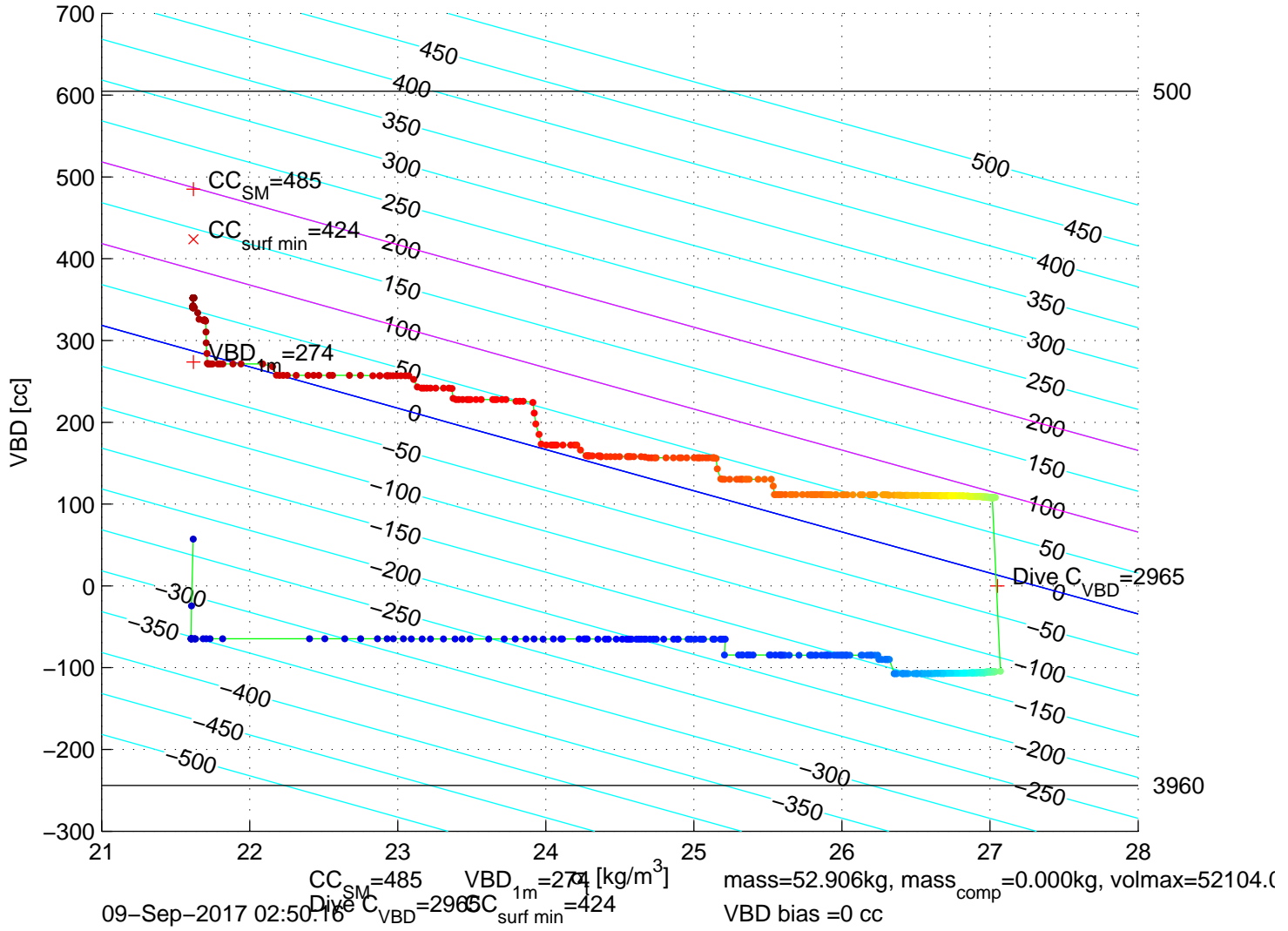
p6100379: SG610 Mission 7 Jul 2017 09-Sep-2017 04:15:56Z – buoyancy contoured
