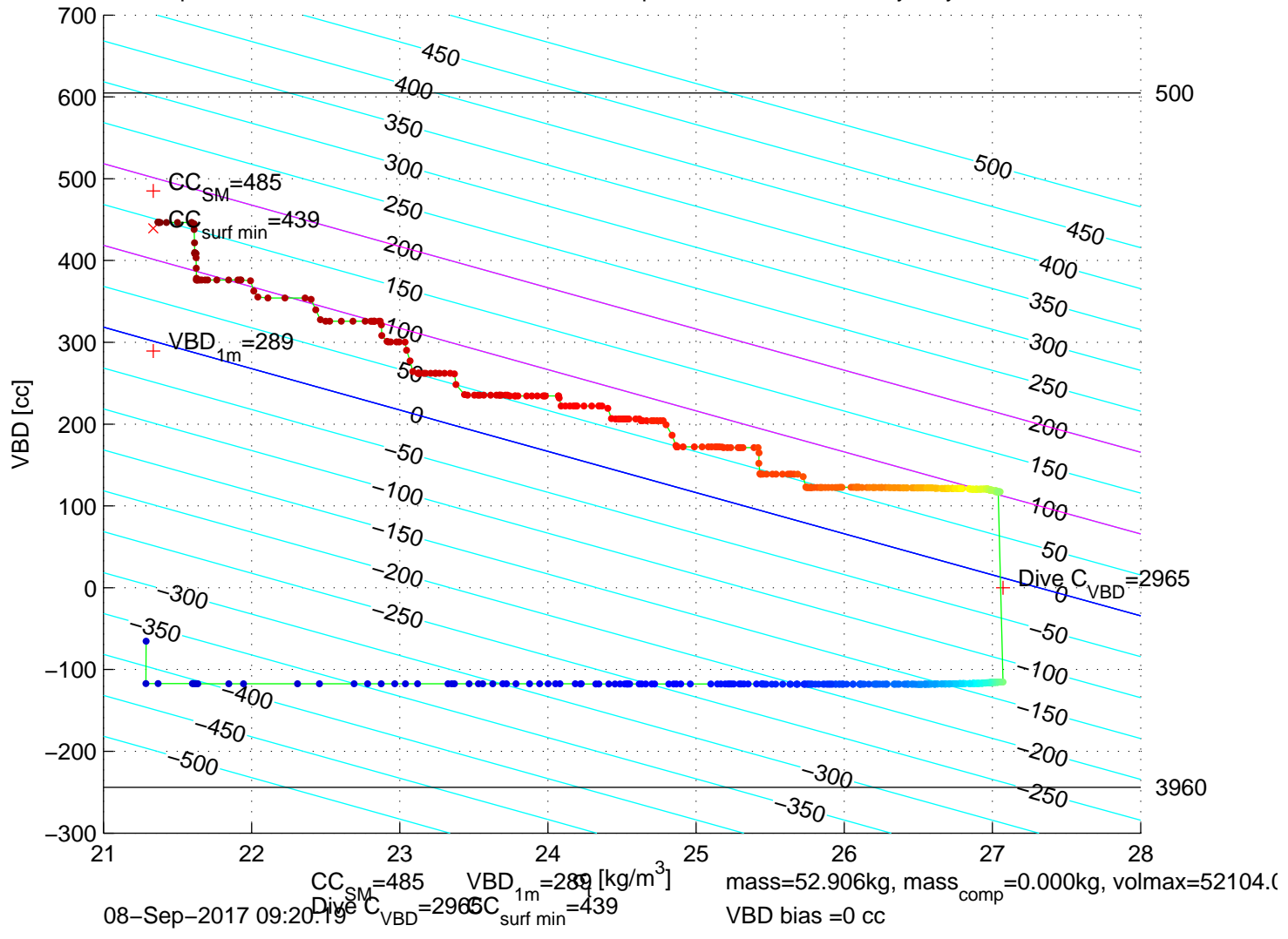
p6100372: SG610 Mission 7 Jul 2017 08-Sep-2017 10:36:47Z – buoyancy contoured
