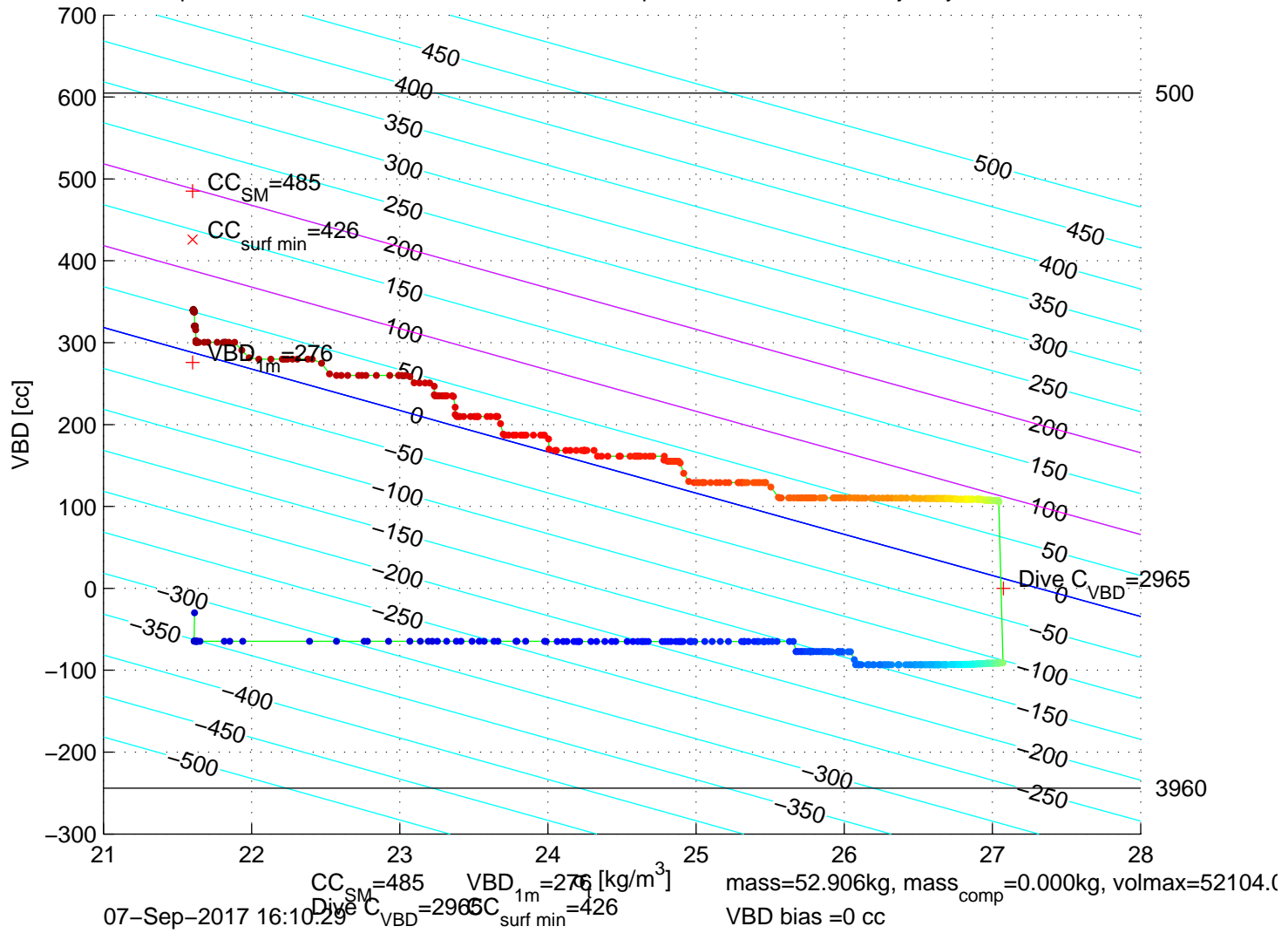
p6100365: SG610 Mission 7 Jul 2017 07-Sep-2017 17:37:25Z – buoyancy contoured
