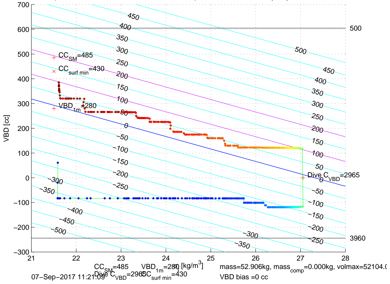
p6100363: SG610 Mission 7 Jul 2017 07-Sep-2017 12:45:44Z – buoyancy contoured
