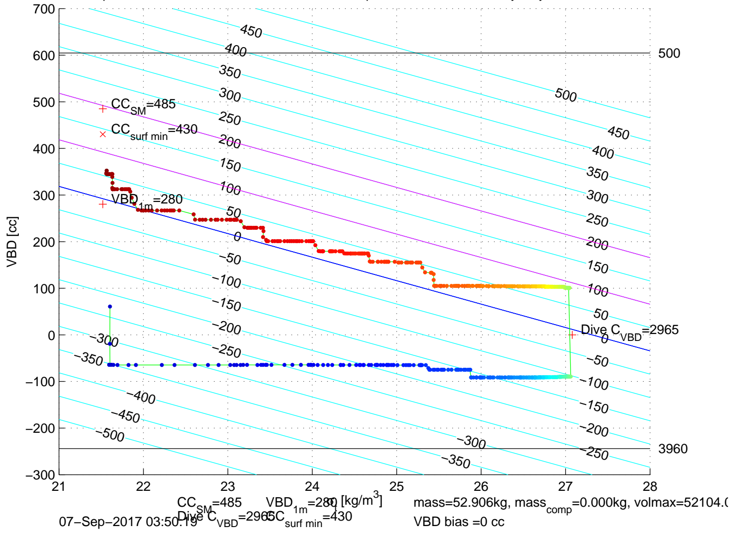
p6100360: SG610 Mission 7 Jul 2017 07-Sep-2017 05:13:48Z – buoyancy contoured
