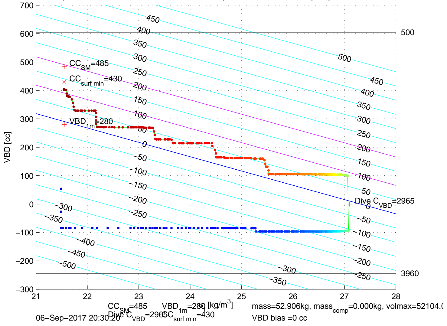
p6100357: SG610 Mission 7 Jul 2017 06-Sep-2017 21:47:31Z – buoyancy contoured
