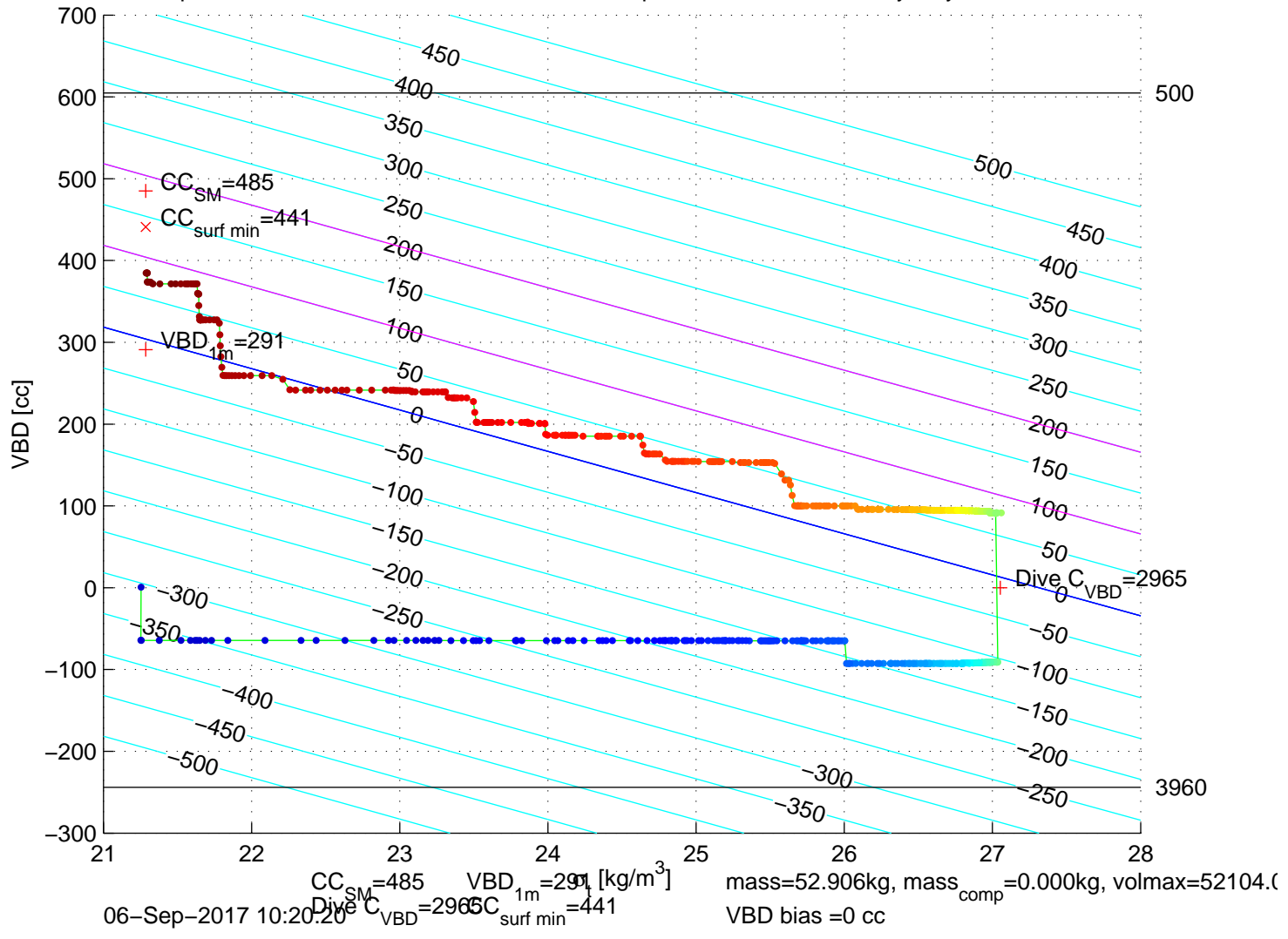
p6100353: SG610 Mission 7 Jul 2017 06-Sep-2017 11:46:23Z – buoyancy contoured
