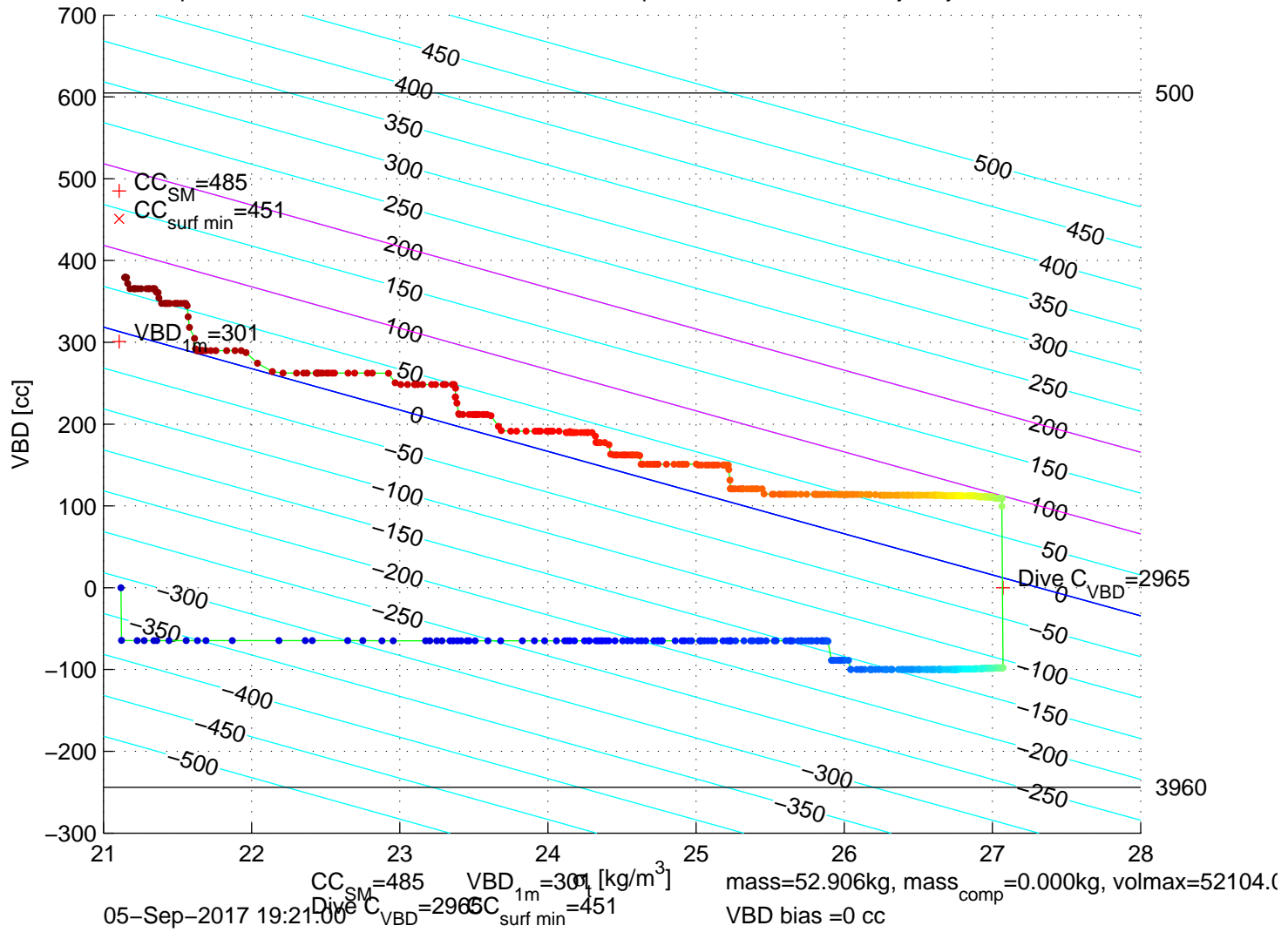
p6100347: SG610 Mission 7 Jul 2017 05-Sep-2017 20:48:04Z – buoyancy contoured
