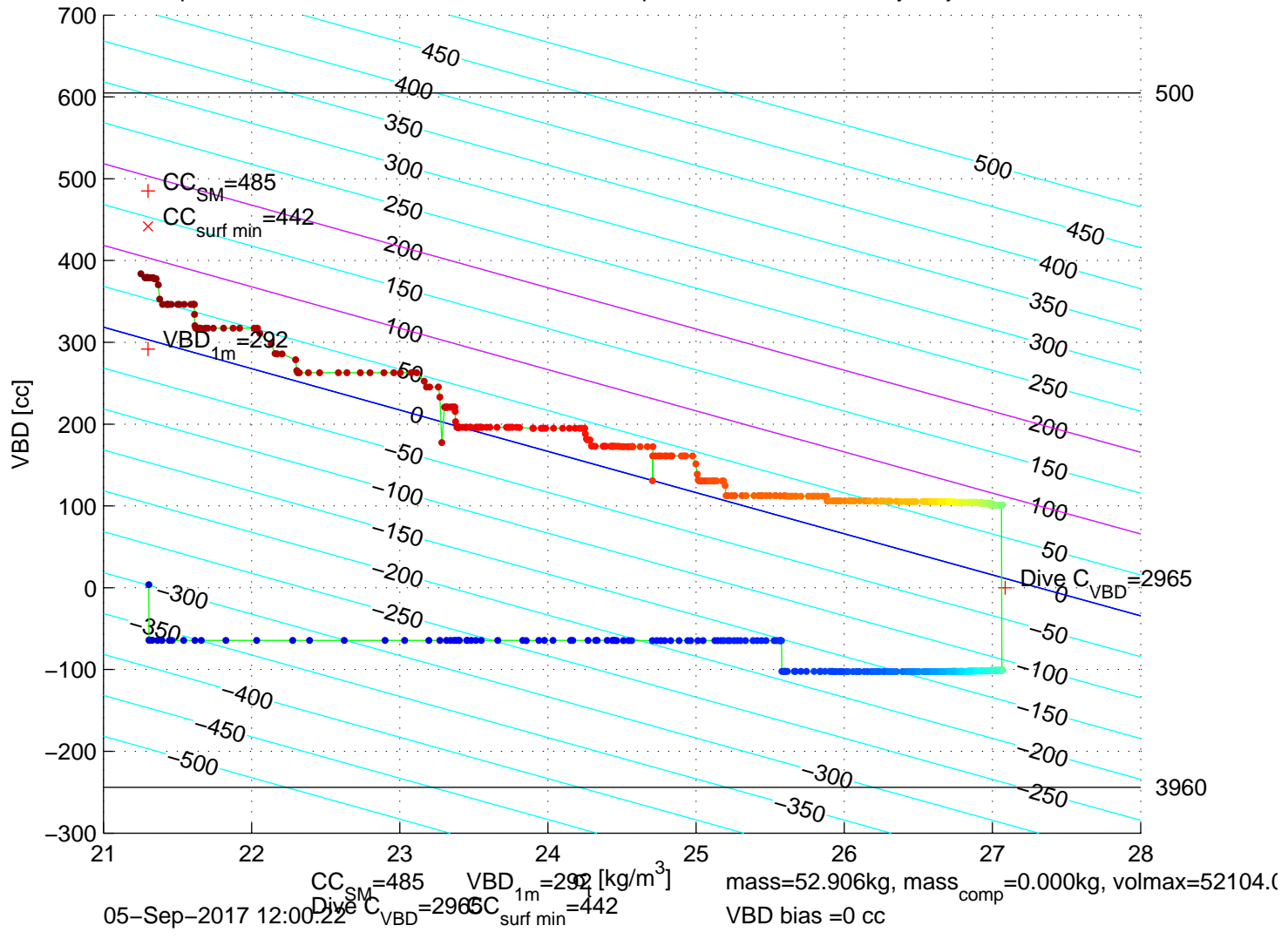
p6100344: SG610 Mission 7 Jul 2017 05-Sep-2017 13:31:20Z – buoyancy contoured
