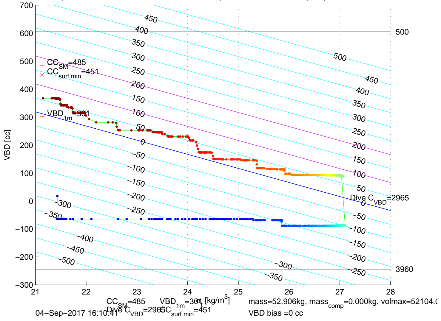
p6100336: SG610 Mission 7 Jul 2017 04-Sep-2017 17:30:29Z – buoyancy contoured
