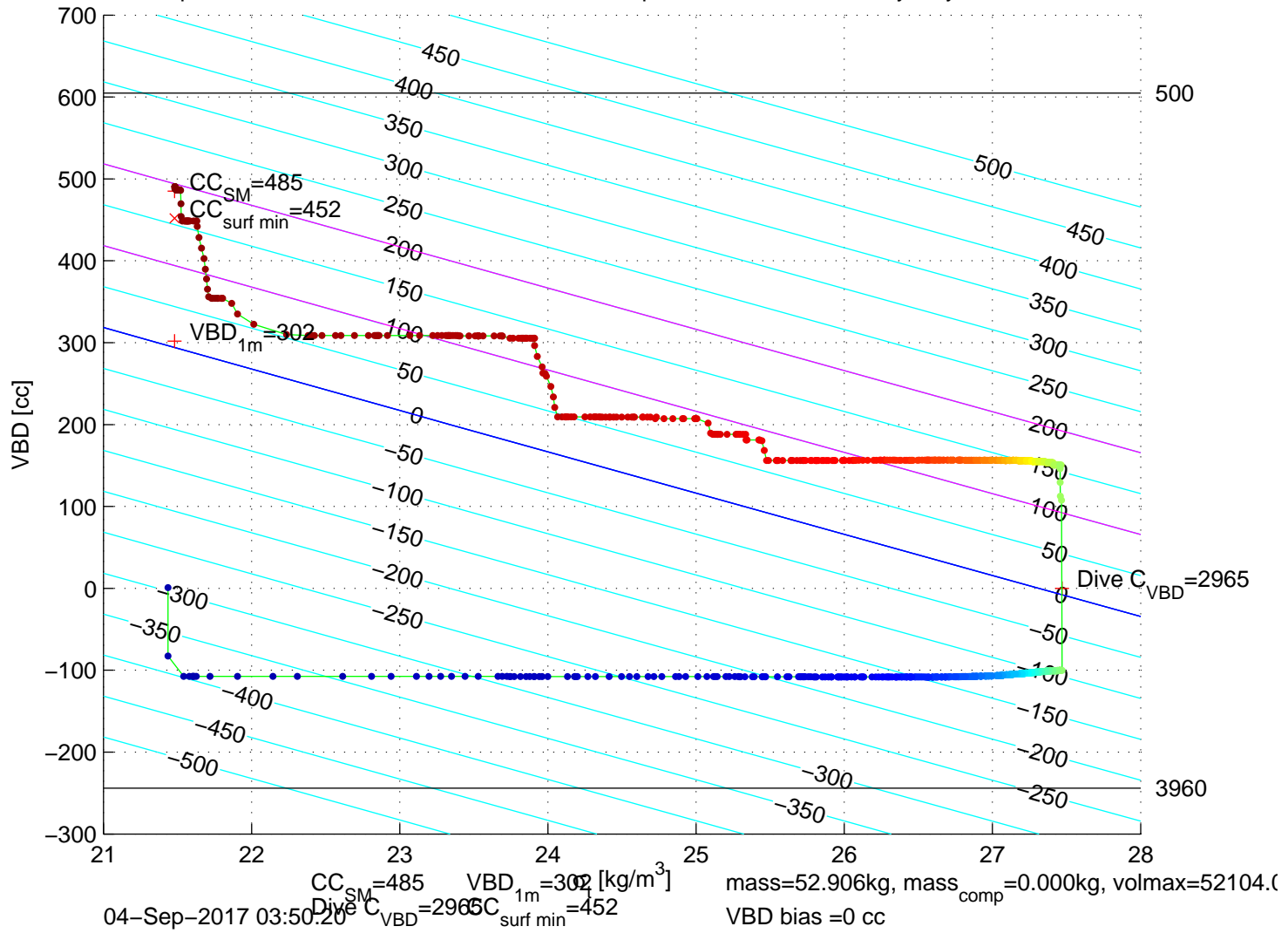
p6100332: SG610 Mission 7 Jul 2017 04-Sep-2017 03:18:14Z – buoyancy contoured
